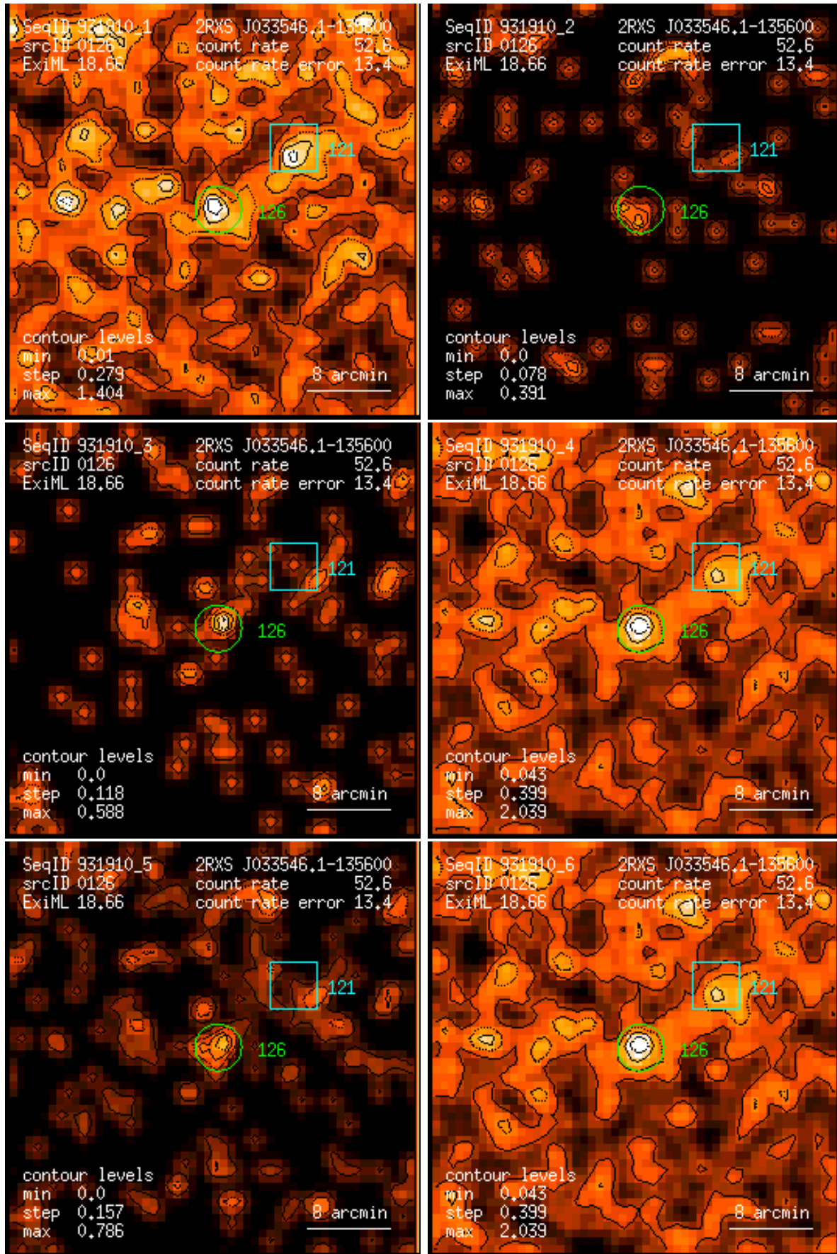
Figure 126: RASS 931910: detection 0126: band rate images, Gaussian filter: (1) PSPC channels 11 – 41, (2) 52 – 90, (3) 91 – 201, (4) 11 – 235, (5) 52 – 201, (6) 11 – 201. Broad band rates in counts/ks. Band rate contour levels in counts/ks/arcmin 2 .
