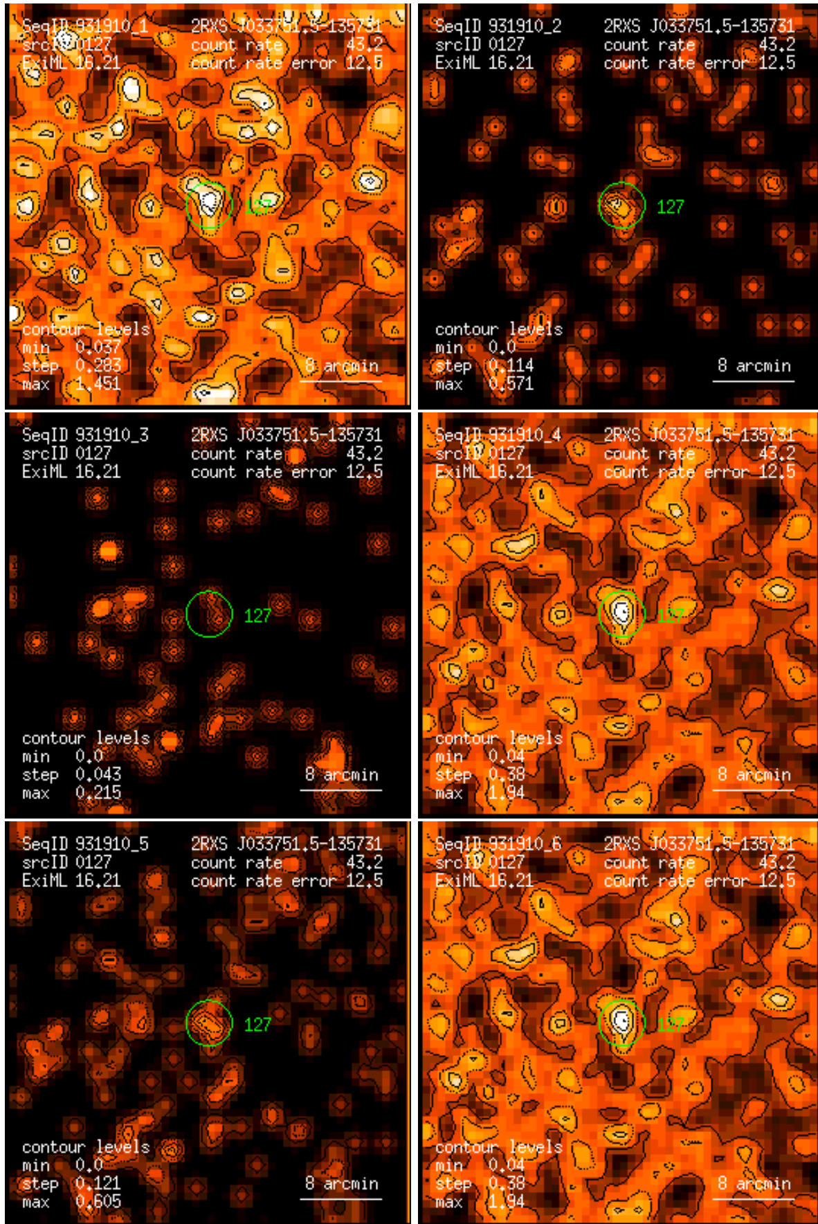
Figure 127: RASS 931910: detection 0127: band rate images, Gaussian filter: (1) PSPC channels 11 – 41, (2) 52 – 90, (3) 91 – 201, (4) 11 – 235, (5) 52 – 201, (6) 11 – 201. Broad band rates in counts/ks. Band rate contour levels in counts/ks/arcmin 2 .
