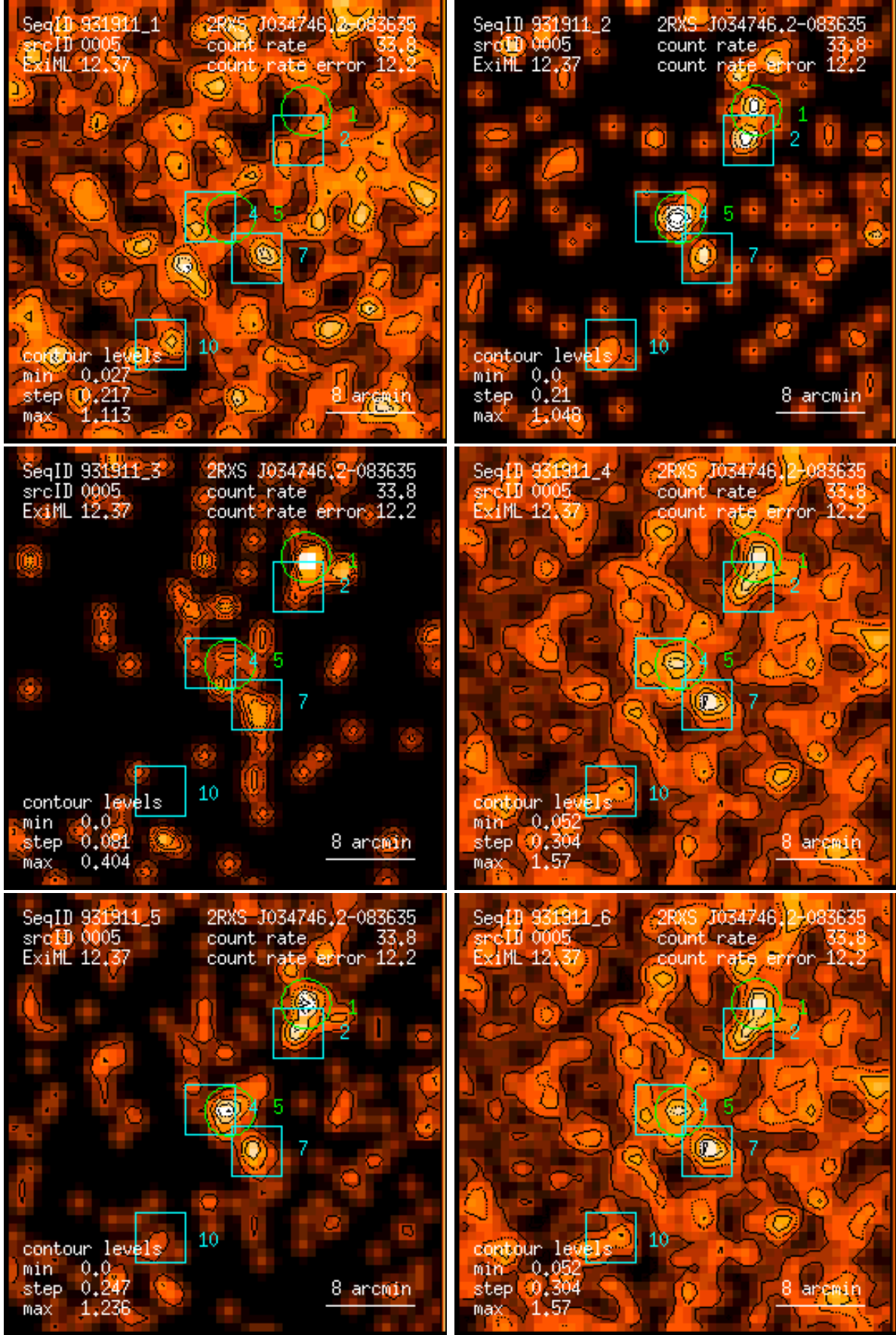
Figure 5: RASS 931911: detection 0005: band rate images, Gaussian filter: (1) PSPC channels 11 – 41, (2) 52 – 90, (3) 91 – 201, (4) 11 – 235, (5) 52 – 201, (6) 11 – 201. Broad band rates in counts/ks. Band rate contour levels in counts/ks/arcmin 2 .
