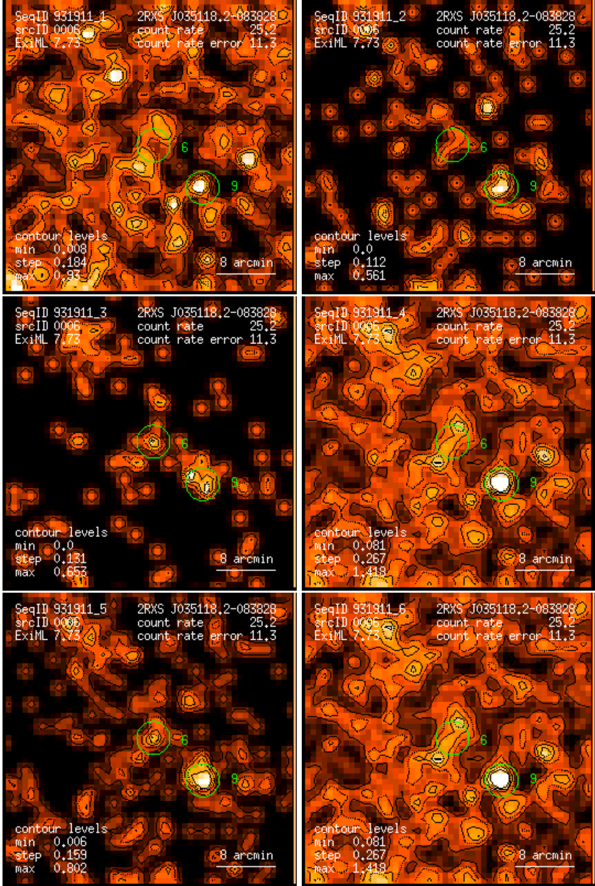
Figure 6: RASS 931911: detection 0006: band rate images, Gaussian filter: (1) PSPC channels 11 – 41, (2) 52 – 90, (3) 91 – 201, (4) 11 – 235, (5) 52 – 201, (6) 11 – 201. Broad band rates in counts/ks. Band rate contour levels in counts/ks/arcmin 2 .
