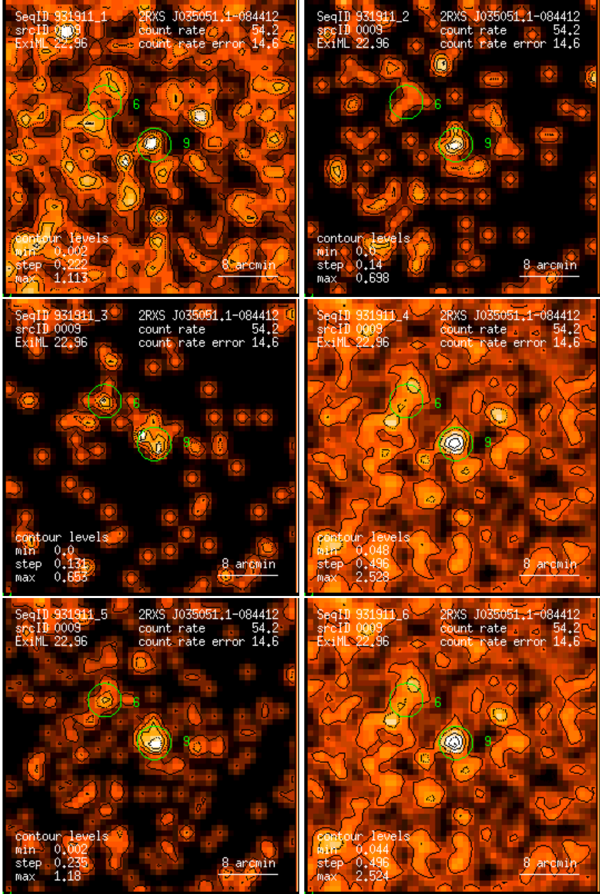
Figure 9: RASS 931911: detection 0009: band rate images, Gaussian filter: (1) PSPC channels 11 – 41, (2) 52 – 90, (3) 91 – 201, (4) 11 – 235, (5) 52 – 201, (6) 11 – 201. Broad band rates in counts/ks. Band rate contour levels in counts/ks/arcmin 2 .
