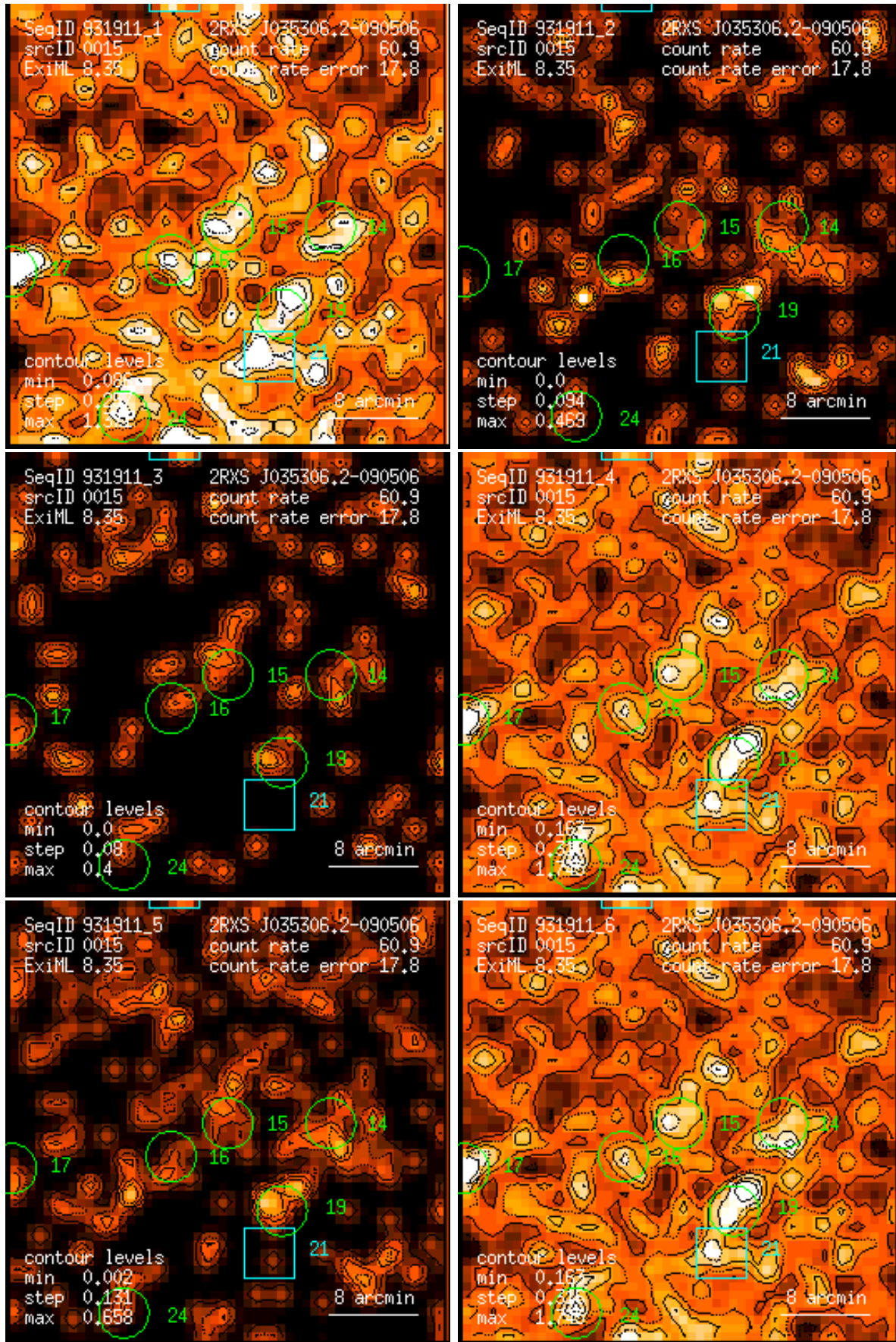
Figure 15: RASS 931911: detection 0015: band rate images, Gaussian filter: (1) PSPC channels 11 – 41, (2) 52 – 90, (3) 91 – 201, (4) 11 – 235, (5) 52 – 201, (6) 11 – 201. Broad band rates in counts/ks. Band rate contour levels in counts/ks/arcmin 2 .
