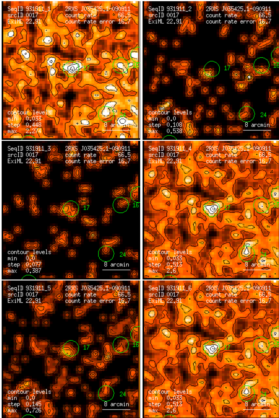
Figure 17: RASS 931911: detection 0017: band rate images, Gaussian filter: (1) PSPC channels 11 – 41, (2) 52 – 90, (3) 91 – 201, (4) 11 – 235, (5) 52 – 201, (6) 11 – 201. Broad band rates in counts/ks. Band rate contour levels in counts/ks/arcmin 2 .
