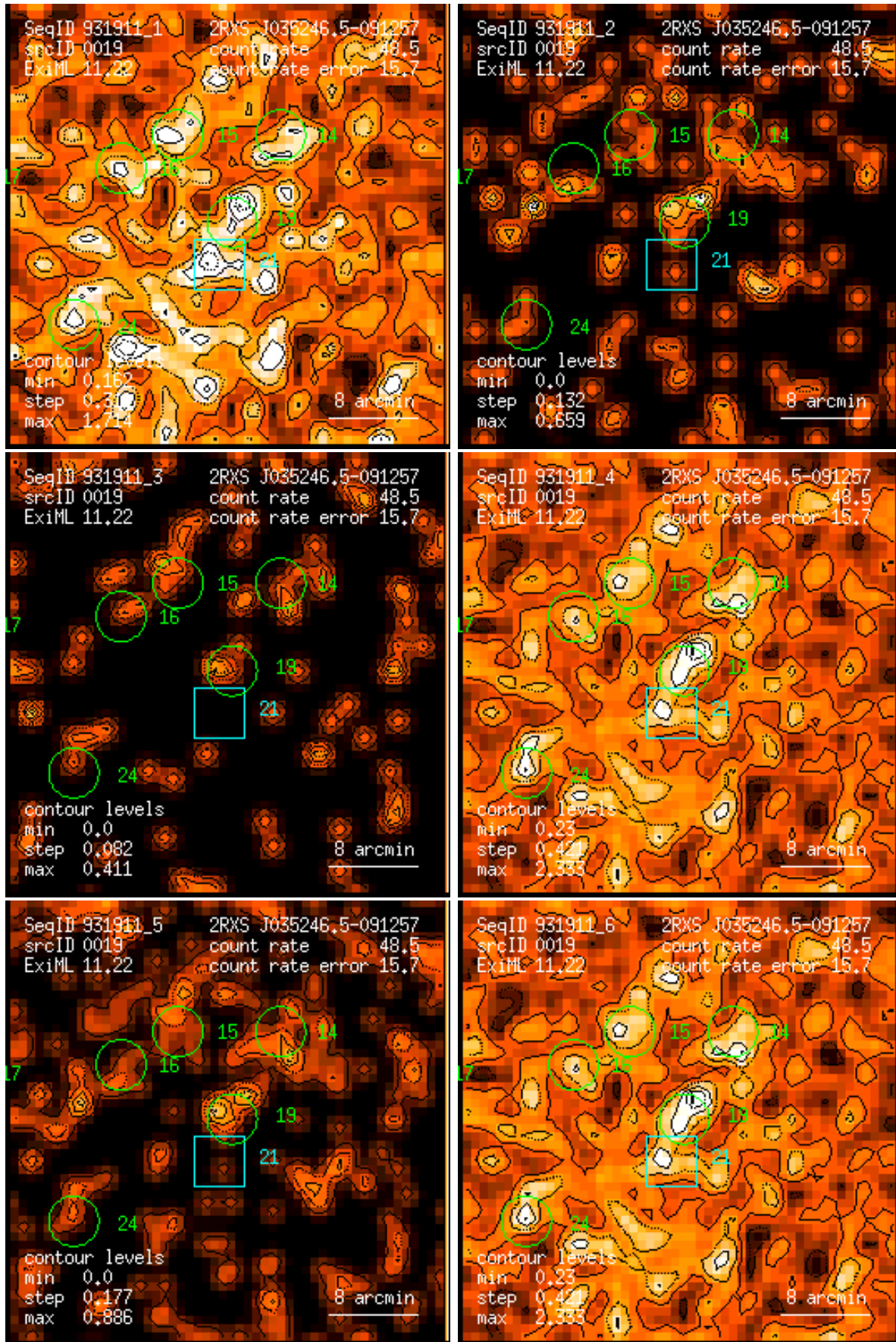
Figure 19: RASS 931911: detection 0019: band rate images, Gaussian filter: (1) PSPC channels 11 – 41, (2) 52 – 90, (3) 91 – 201, (4) 11 – 235, (5) 52 – 201, (6) 11 – 201. Broad band rates in counts/ks. Band rate contour levels in counts/ks/arcmin 2 .
