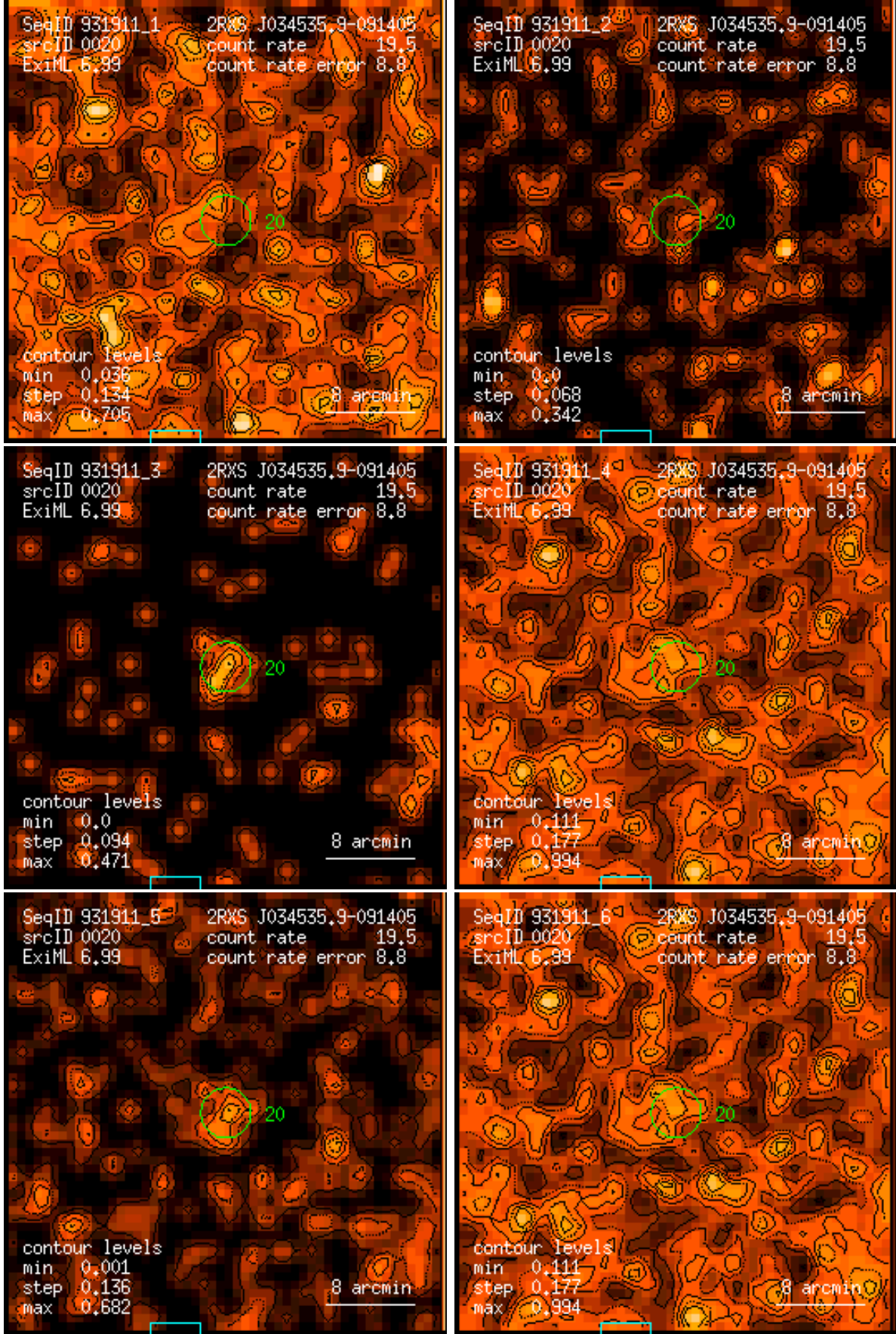
Figure 20: RASS 931911: detection 0020: band rate images, Gaussian filter: (1) PSPC channels 11 – 41, (2) 52 – 90, (3) 91 – 201, (4) 11 – 235, (5) 52 – 201, (6) 11 – 201. Broad band rates in counts/ks. Band rate contour levels in counts/ks/arcmin 2 .
