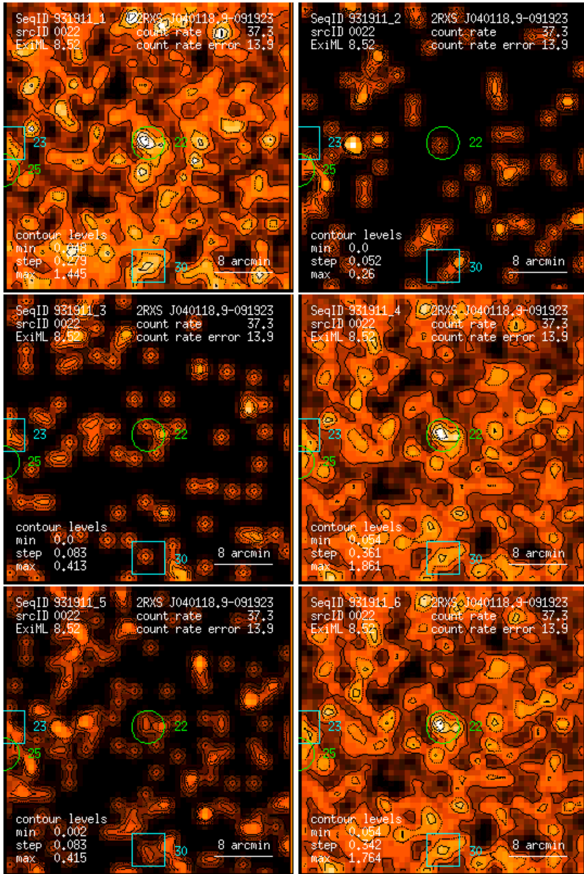
Figure 22: RASS 931911: detection 0022: band rate images, Gaussian filter: (1) PSPC channels 11 – 41, (2) 52 – 90, (3) 91 – 201, (4) 11 – 235, (5) 52 – 201, (6) 11 – 201. Broad band rates in counts/ks. Band rate contour levels in counts/ks/arcmin 2 .
