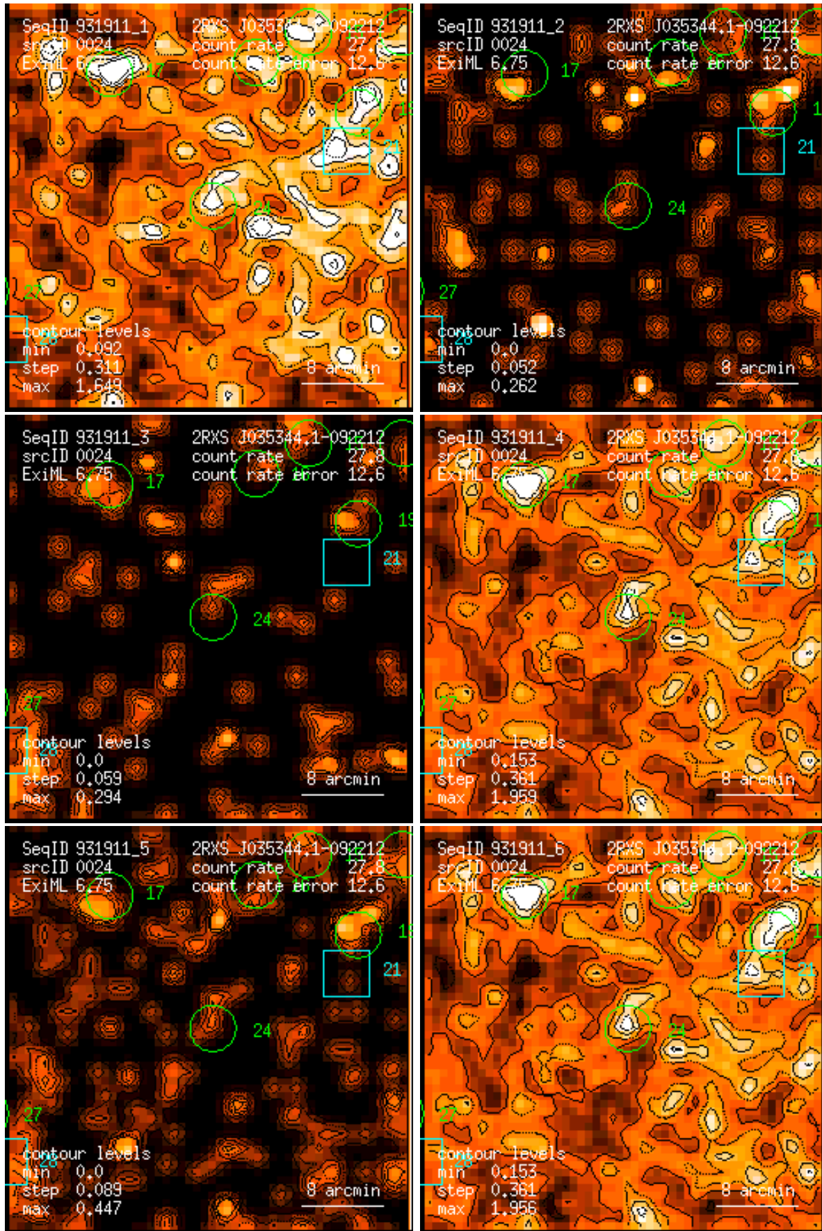
Figure 24: RASS 931911: detection 0024: band rate images, Gaussian filter: (1) PSPC channels 11 – 41, (2) 52 – 90, (3) 91 – 201, (4) 11 – 235, (5) 52 – 201, (6) 11 – 201. Broad band rates in counts/ks. Band rate contour levels in counts/ks/arcmin 2 .
