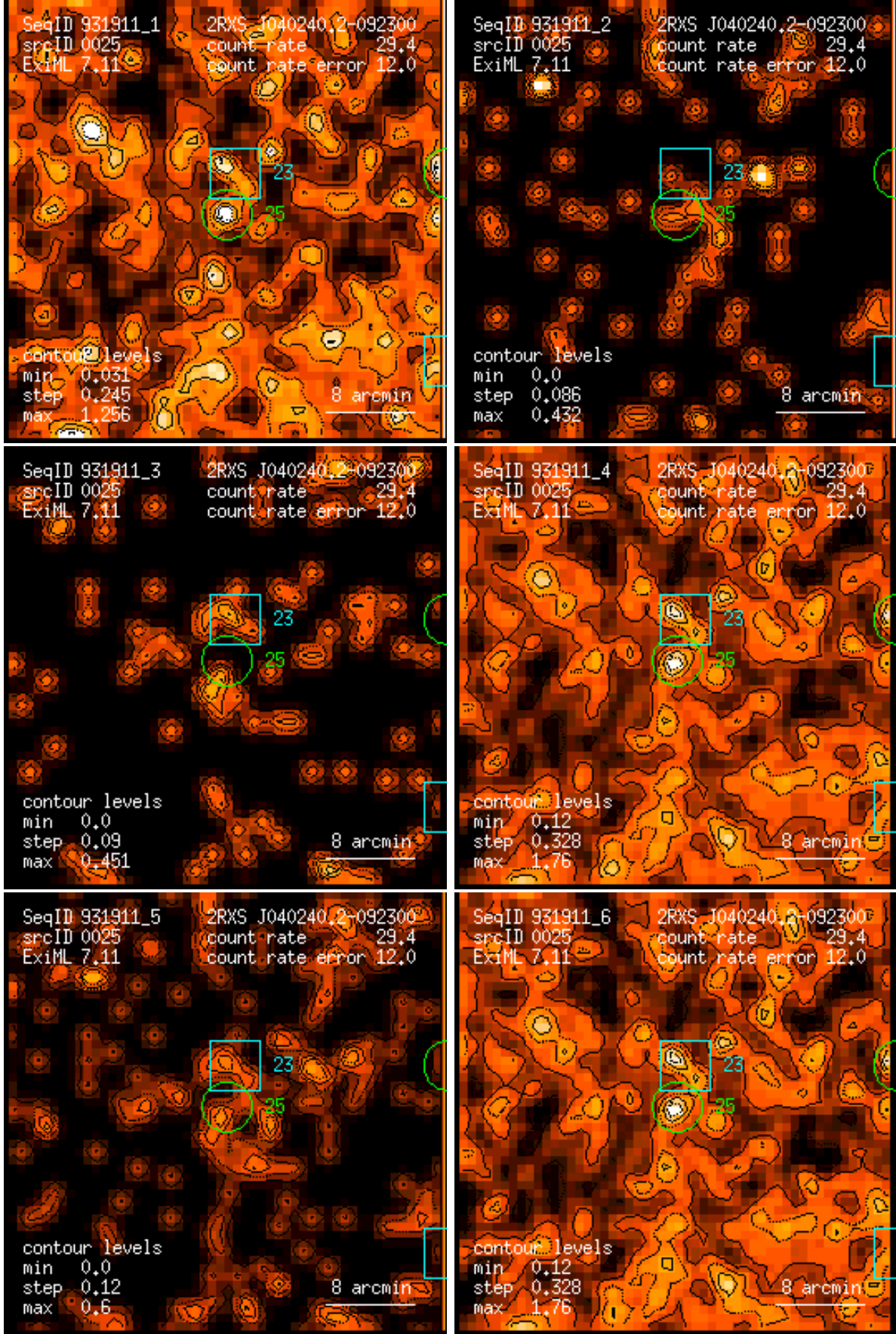
Figure 25: RASS 931911: detection 0025: band rate images, Gaussian filter: (1) PSPC channels 11 – 41, (2) 52 – 90, (3) 91 – 201, (4) 11 – 235, (5) 52 – 201, (6) 11 – 201. Broad band rates in counts/ks. Band rate contour levels in counts/ks/arcmin 2 .
