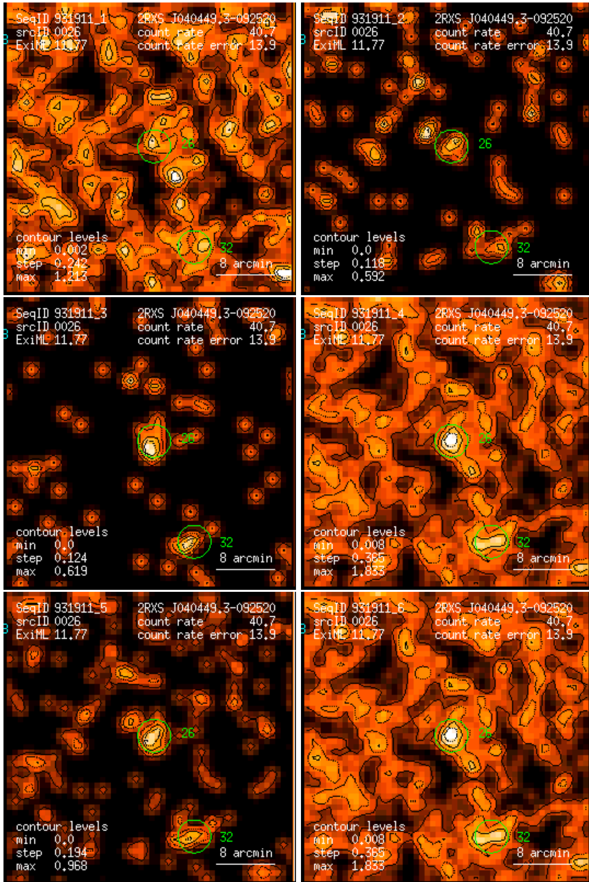
Figure 26: RASS 931911: detection 0026: band rate images, Gaussian filter: (1) PSPC channels 11 – 41, (2) 52 – 90, (3) 91 – 201, (4) 11 – 235, (5) 52 – 201, (6) 11 – 201. Broad band rates in counts/ks. Band rate contour levels in counts/ks/arcmin 2 .
