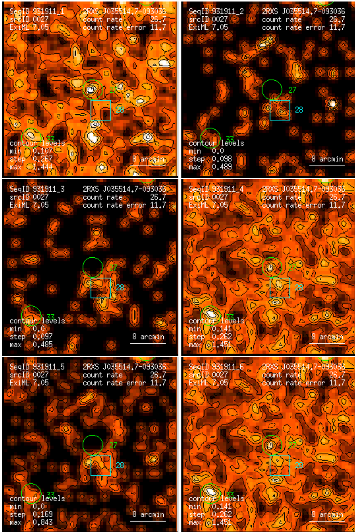
Figure 27: RASS 931911: detection 0027: band rate images, Gaussian filter: (1) PSPC channels 11 – 41, (2) 52 – 90, (3) 91 – 201, (4) 11 – 235, (5) 52 – 201, (6) 11 – 201. Broad band rates in counts/ks. Band rate contour levels in counts/ks/arcmin 2 .
