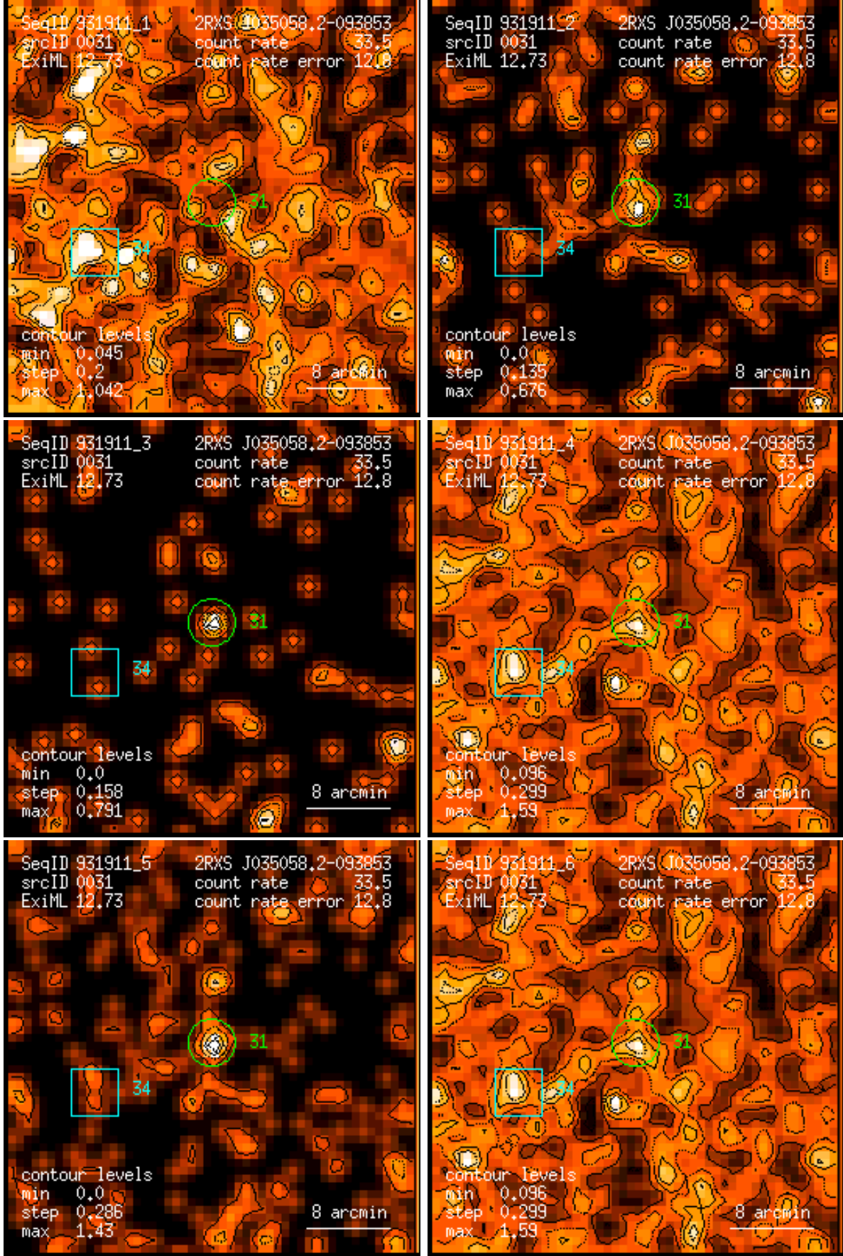
Figure 31: RASS 931911: detection 0031: band rate images, Gaussian filter: (1) PSPC channels 11 – 41, (2) 52 – 90, (3) 91 – 201, (4) 11 – 235, (5) 52 – 201, (6) 11 – 201. Broad band rates in counts/ks. Band rate contour levels in counts/ks/arcmin 2 .
