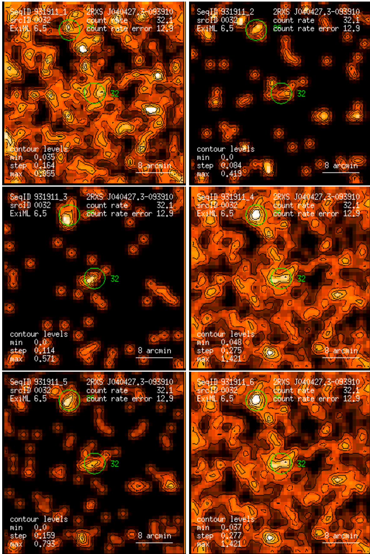
Figure 32: RASS 931911: detection 0032: band rate images, Gaussian filter: (1) PSPC channels 11 – 41, (2) 52 – 90, (3) 91 – 201, (4) 11 – 235, (5) 52 – 201, (6) 11 – 201. Broad band rates in counts/ks. Band rate contour levels in counts/ks/arcmin 2 .
