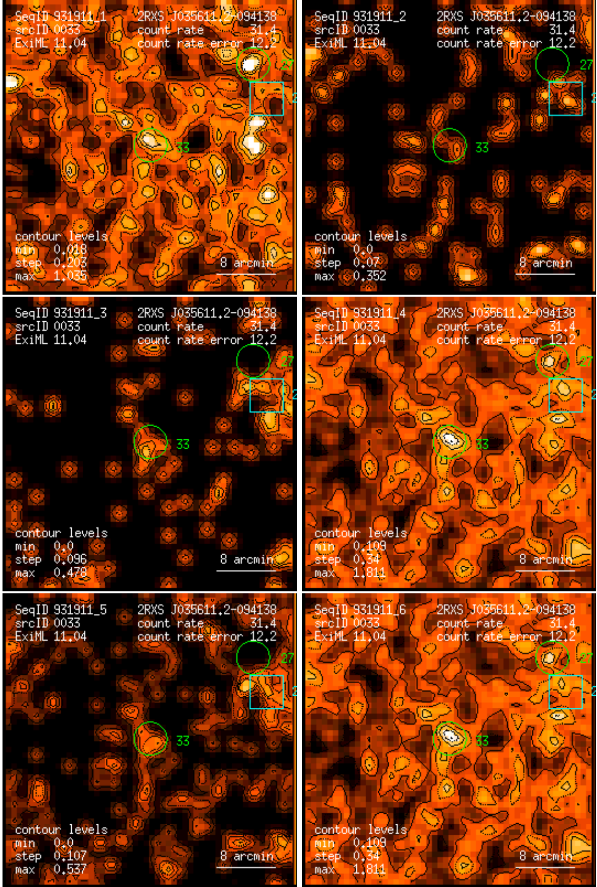
Figure 33: RASS 931911: detection 0033: band rate images, Gaussian filter: (1) PSPC channels 11 – 41, (2) 52 – 90, (3) 91 – 201, (4) 11 – 235, (5) 52 – 201, (6) 11 – 201. Broad band rates in counts/ks. Band rate contour levels in counts/ks/arcmin 2 .
