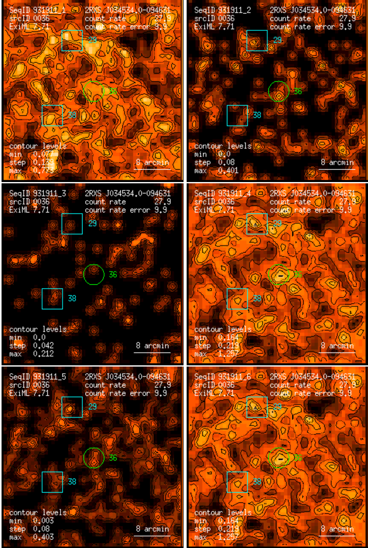
Figure 36: RASS 931911: detection 0036: band rate images, Gaussian filter: (1) PSPC channels 11 – 41, (2) 52 – 90, (3) 91 – 201, (4) 11 – 235, (5) 52 – 201, (6) 11 – 201. Broad band rates in counts/ks. Band rate contour levels in counts/ks/arcmin 2 .
