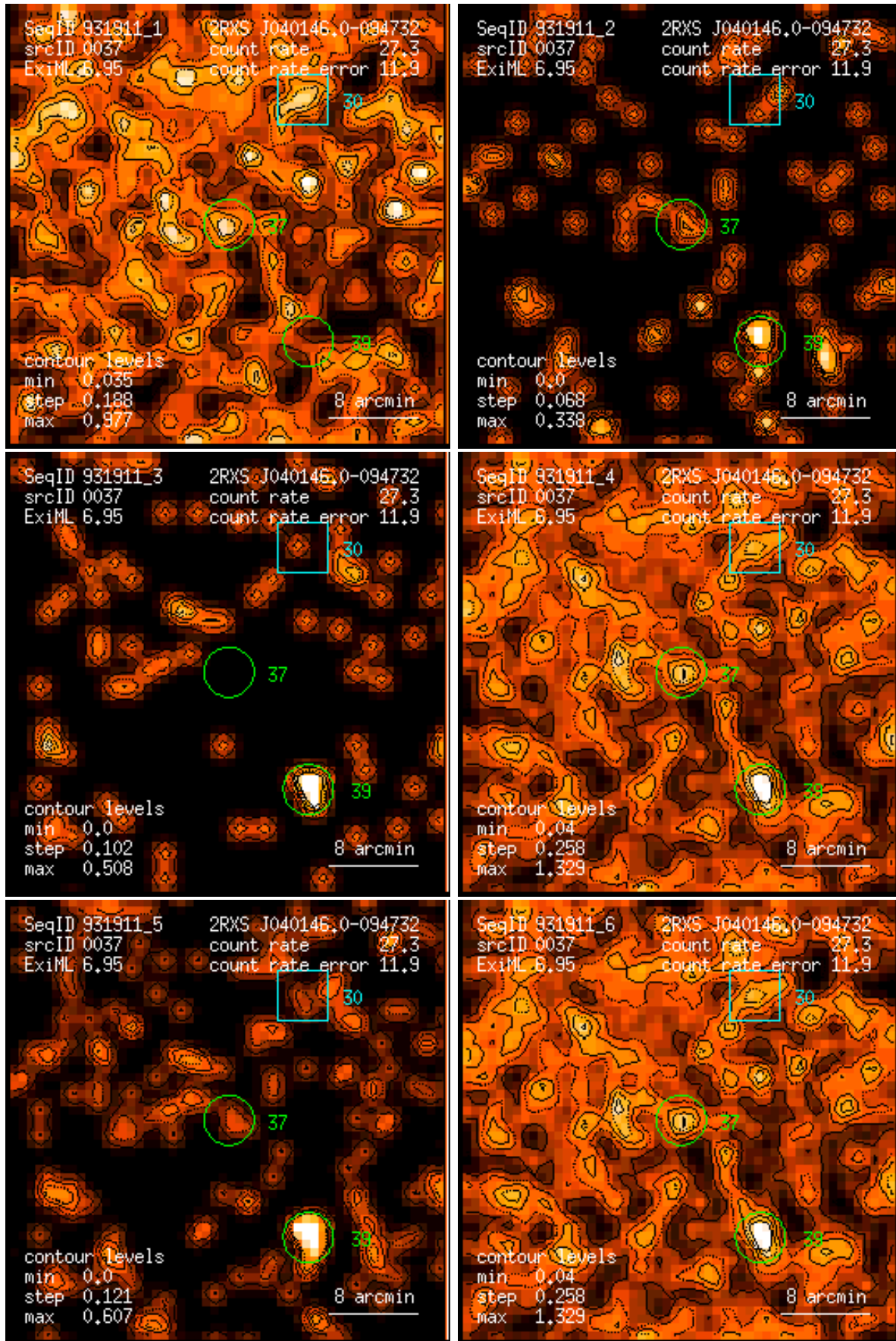
Figure 37: RASS 931911: detection 0037: band rate images, Gaussian filter: (1) PSPC channels 11 – 41, (2) 52 – 90, (3) 91 – 201, (4) 11 – 235, (5) 52 – 201, (6) 11 – 201. Broad band rates in counts/ks. Band rate contour levels in counts/ks/arcmin 2 .
