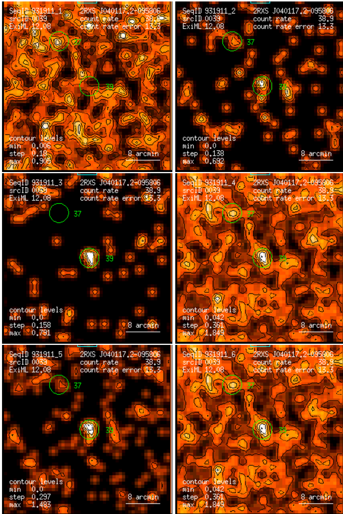
Figure 39: RASS 931911: detection 0039: band rate images, Gaussian filter: (1) PSPC channels 11 – 41, (2) 52 – 90, (3) 91 – 201, (4) 11 – 235, (5) 52 – 201, (6) 11 – 201. Broad band rates in counts/ks. Band rate contour levels in counts/ks/arcmin 2 .
