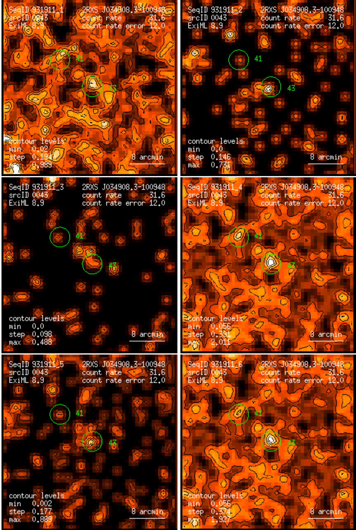
Figure 43: RASS 931911: detection 0043: band rate images, Gaussian filter: (1) PSPC channels 11 – 41, (2) 52 – 90, (3) 91 – 201, (4) 11 – 235, (5) 52 – 201, (6) 11 – 201. Broad band rates in counts/ks. Band rate contour levels in counts/ks/arcmin 2 .
