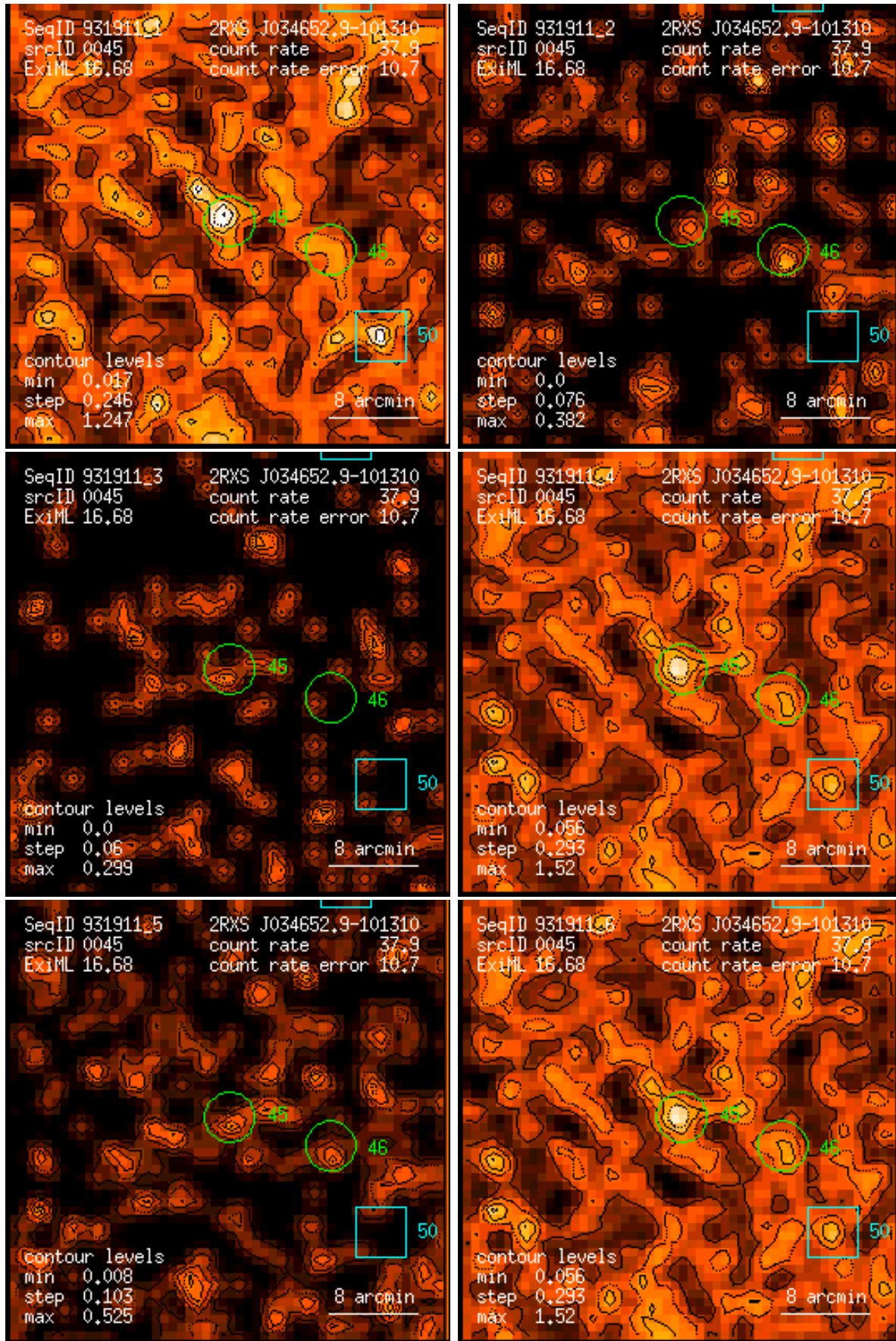
Figure 45: RASS 931911: detection 0045: band rate images, Gaussian filter: (1) PSPC channels 11 – 41, (2) 52 – 90, (3) 91 – 201, (4) 11 – 235, (5) 52 – 201, (6) 11 – 201. Broad band rates in counts/ks. Band rate contour levels in counts/ks/arcmin 2 .
