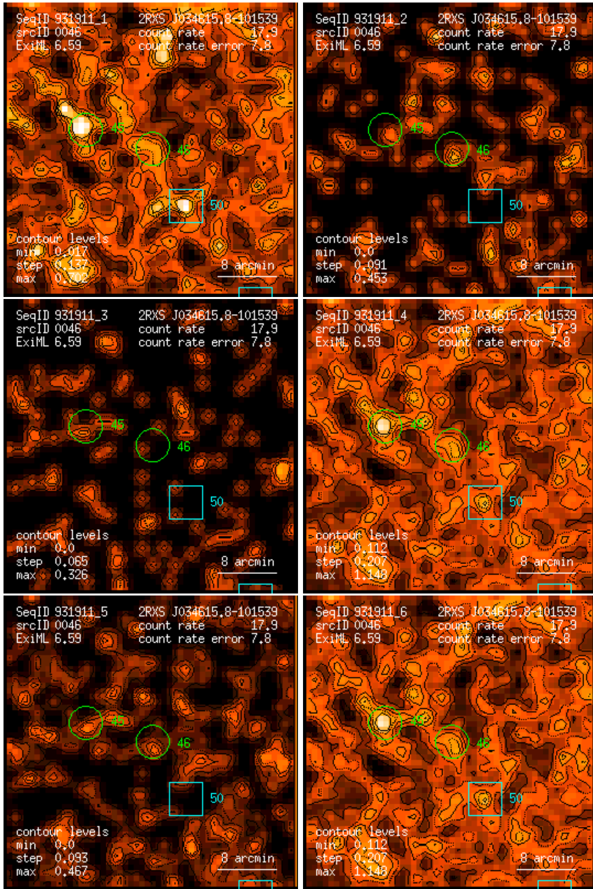
Figure 46: RASS 931911: detection 0046: band rate images, Gaussian filter: (1) PSPC channels 11 – 41, (2) 52 – 90, (3) 91 – 201, (4) 11 – 235, (5) 52 – 201, (6) 11 – 201. Broad band rates in counts/ks. Band rate contour levels in counts/ks/arcmin 2 .
