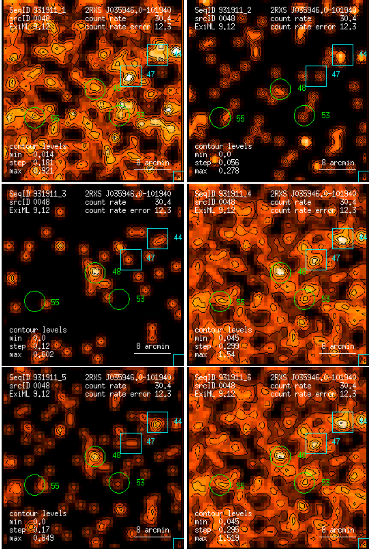
Figure 48: RASS 931911: detection 0048: band rate images, Gaussian filter: (1) PSPC channels 11 – 41, (2) 52 – 90, (3) 91 – 201, (4) 11 – 235, (5) 52 – 201, (6) 11 – 201. Broad band rates in counts/ks. Band rate contour levels in counts/ks/arcmin 2 .
