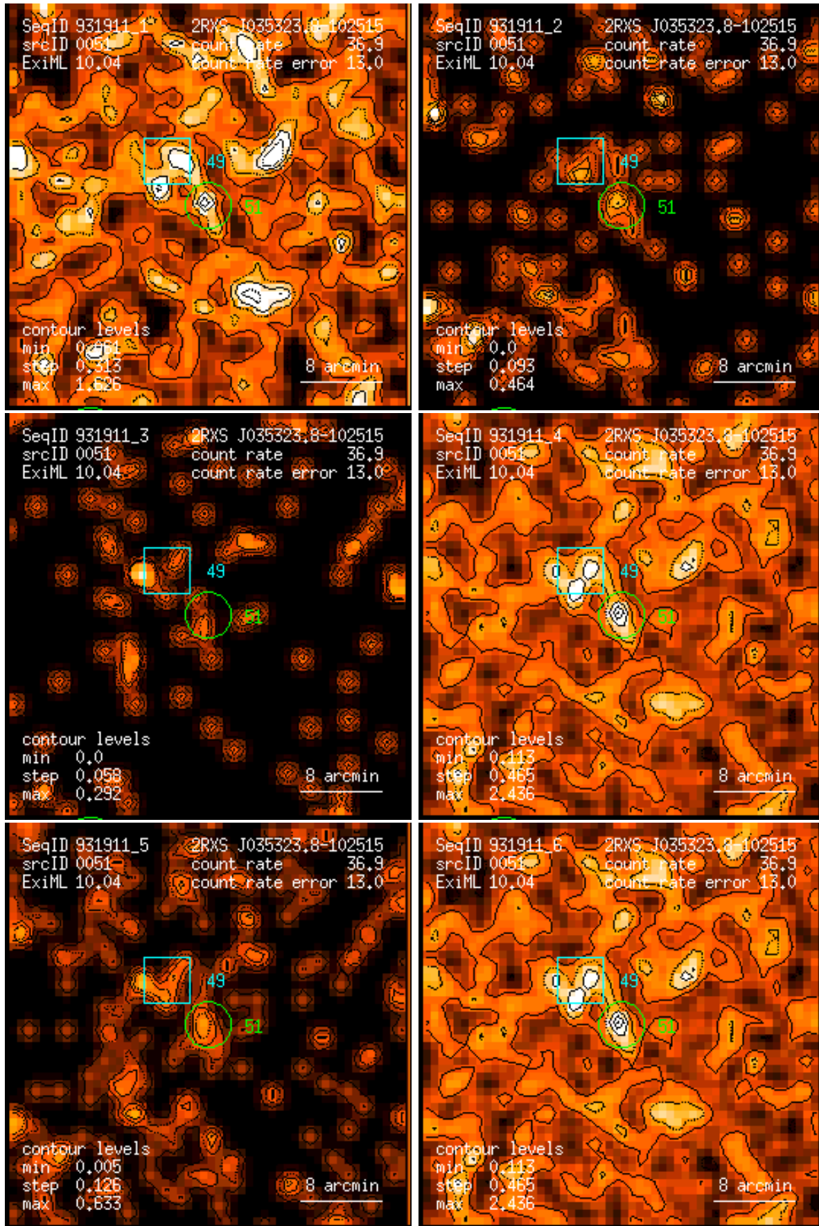
Figure 51: RASS 931911: detection 0051: band rate images, Gaussian filter: (1) PSPC channels 11 – 41, (2) 52 – 90, (3) 91 – 201, (4) 11 – 235, (5) 52 – 201, (6) 11 – 201. Broad band rates in counts/ks. Band rate contour levels in counts/ks/arcmin 2 .
