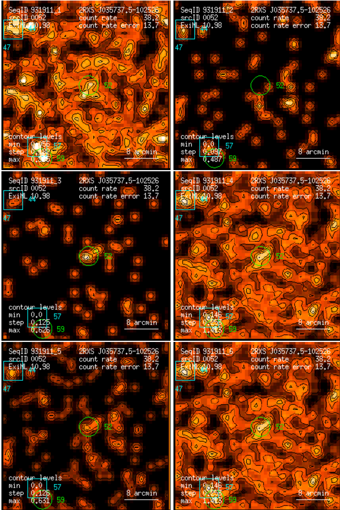
Figure 52: RASS 931911: detection 0052: band rate images, Gaussian filter: (1) PSPC channels 11 – 41, (2) 52 – 90, (3) 91 – 201, (4) 11 – 235, (5) 52 – 201, (6) 11 – 201. Broad band rates in counts/ks. Band rate contour levels in counts/ks/arcmin 2 .
