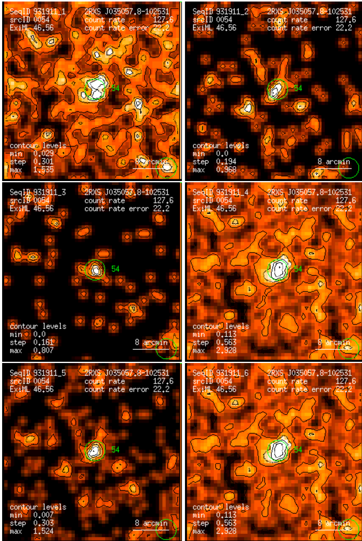
Figure 54: RASS 931911: detection 0054: band rate images, Gaussian filter: (1) PSPC channels 11 – 41, (2) 52 – 90, (3) 91 – 201, (4) 11 – 235, (5) 52 – 201, (6) 11 – 201. Broad band rates in counts/ks. Band rate contour levels in counts/ks/arcmin 2 .
