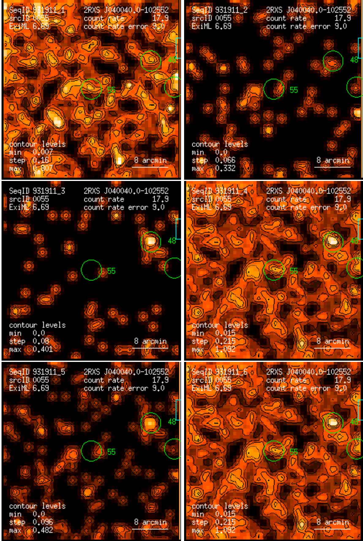
Figure 55: RASS 931911: detection 0055: band rate images, Gaussian filter: (1) PSPC channels 11 – 41, (2) 52 – 90, (3) 91 – 201, (4) 11 – 235, (5) 52 – 201, (6) 11 – 201. Broad band rates in counts/ks. Band rate contour levels in counts/ks/arcmin 2 .
