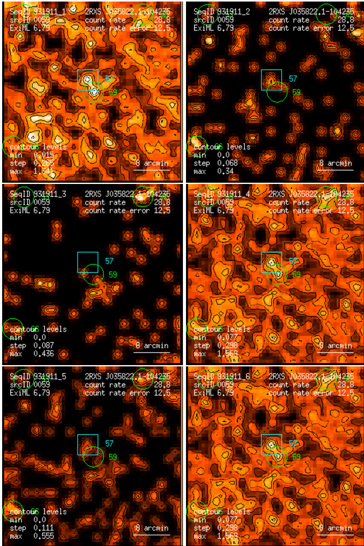
Figure 59: RASS 931911: detection 0059: band rate images, Gaussian filter: (1) PSPC channels 11 – 41, (2) 52 – 90, (3) 91 – 201, (4) 11 – 235, (5) 52 – 201, (6) 11 – 201. Broad band rates in counts/ks. Band rate contour levels in counts/ks/arcmin 2 .
