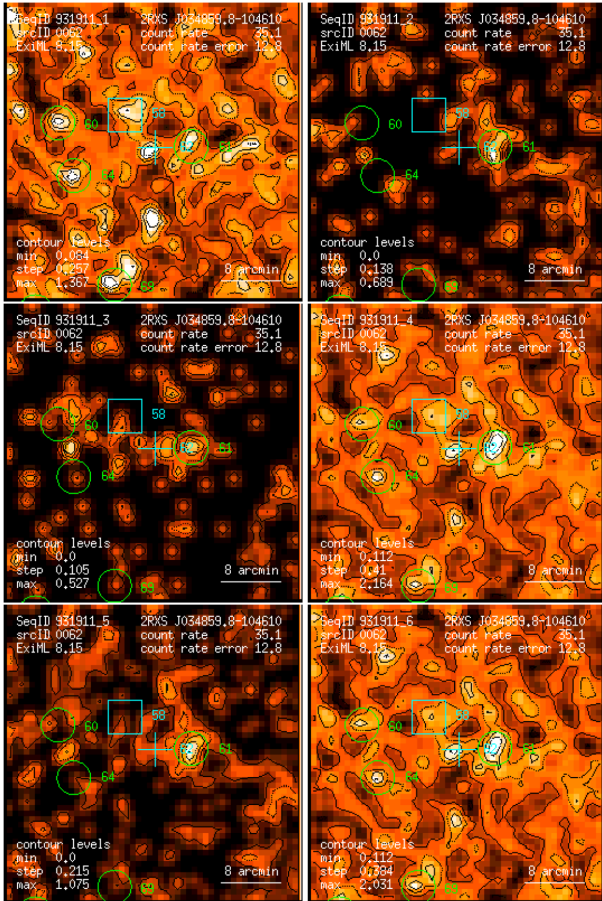
Figure 62: RASS 931911: detection 0062: band rate images, Gaussian filter: (1) PSPC channels 11 – 41, (2) 52 – 90, (3) 91 – 201, (4) 11 – 235, (5) 52 – 201, (6) 11 – 201. Broad band rates in counts/ks. Band rate contour levels in counts/ks/arcmin 2 .
