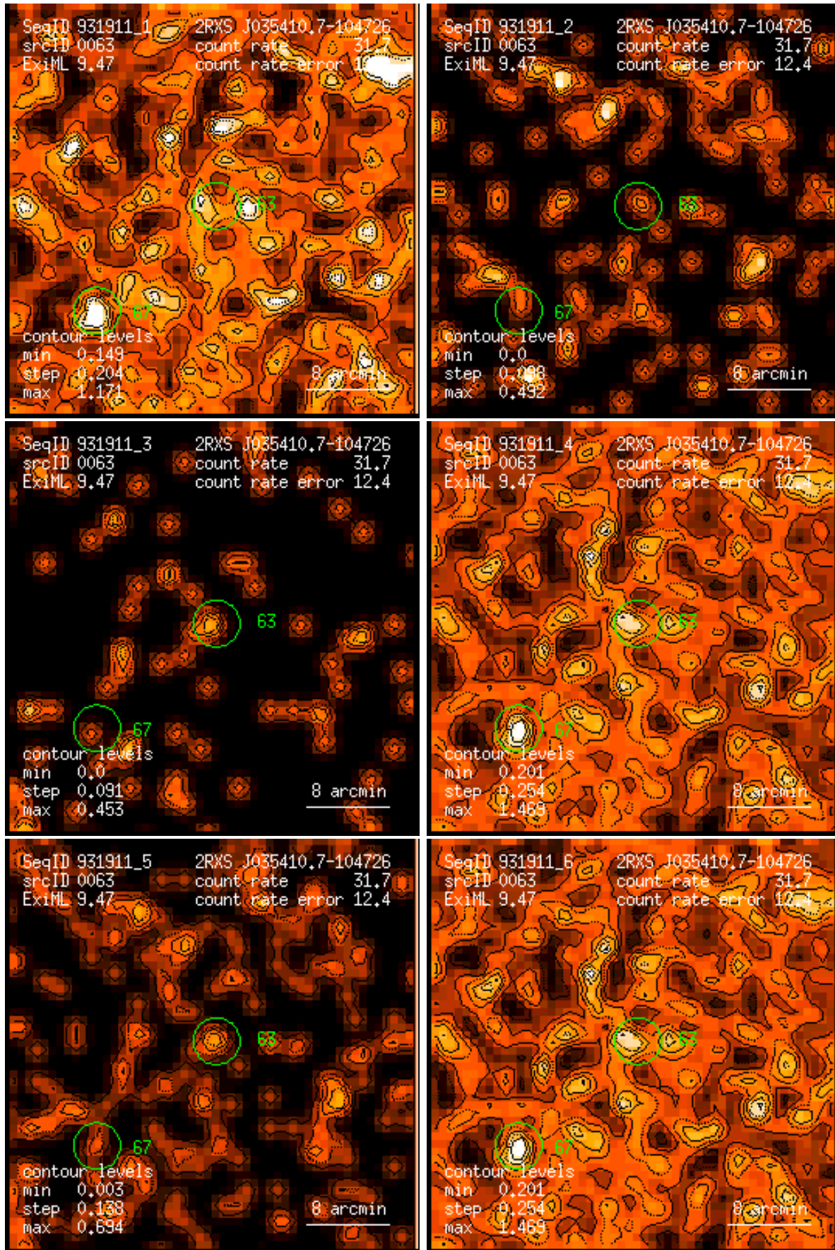
Figure 63: RASS 931911: detection 0063: band rate images, Gaussian filter: (1) PSPC channels 11 – 41, (2) 52 – 90, (3) 91 – 201, (4) 11 – 235, (5) 52 – 201, (6) 11 – 201. Broad band rates in counts/ks. Band rate contour levels in counts/ks/arcmin 2 .
