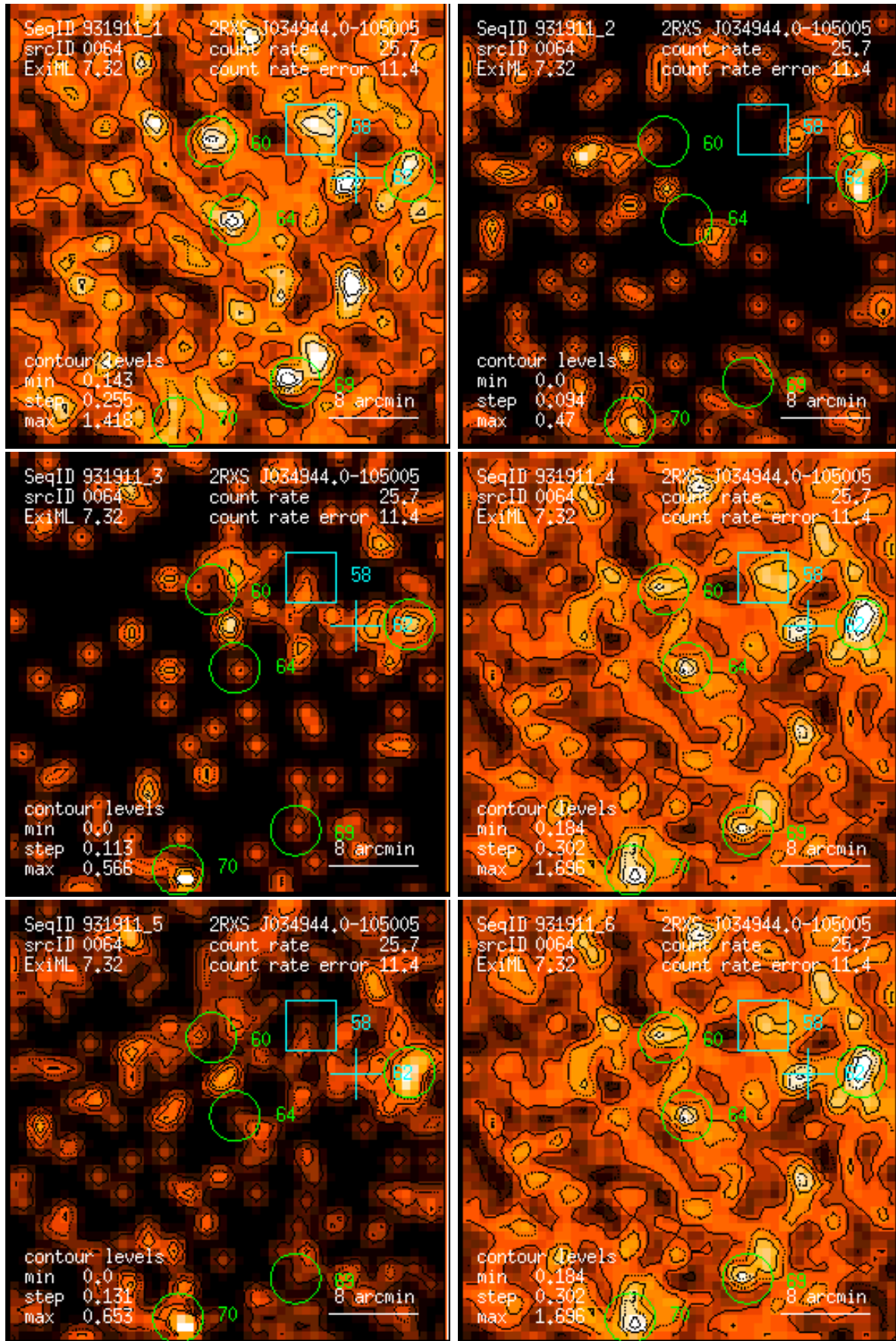
Figure 64: RASS 931911: detection 0064: band rate images, Gaussian filter: (1) PSPC channels 11 – 41, (2) 52 – 90, (3) 91 – 201, (4) 11 – 235, (5) 52 – 201, (6) 11 – 201. Broad band rates in counts/ks. Band rate contour levels in counts/ks/arcmin 2 .
