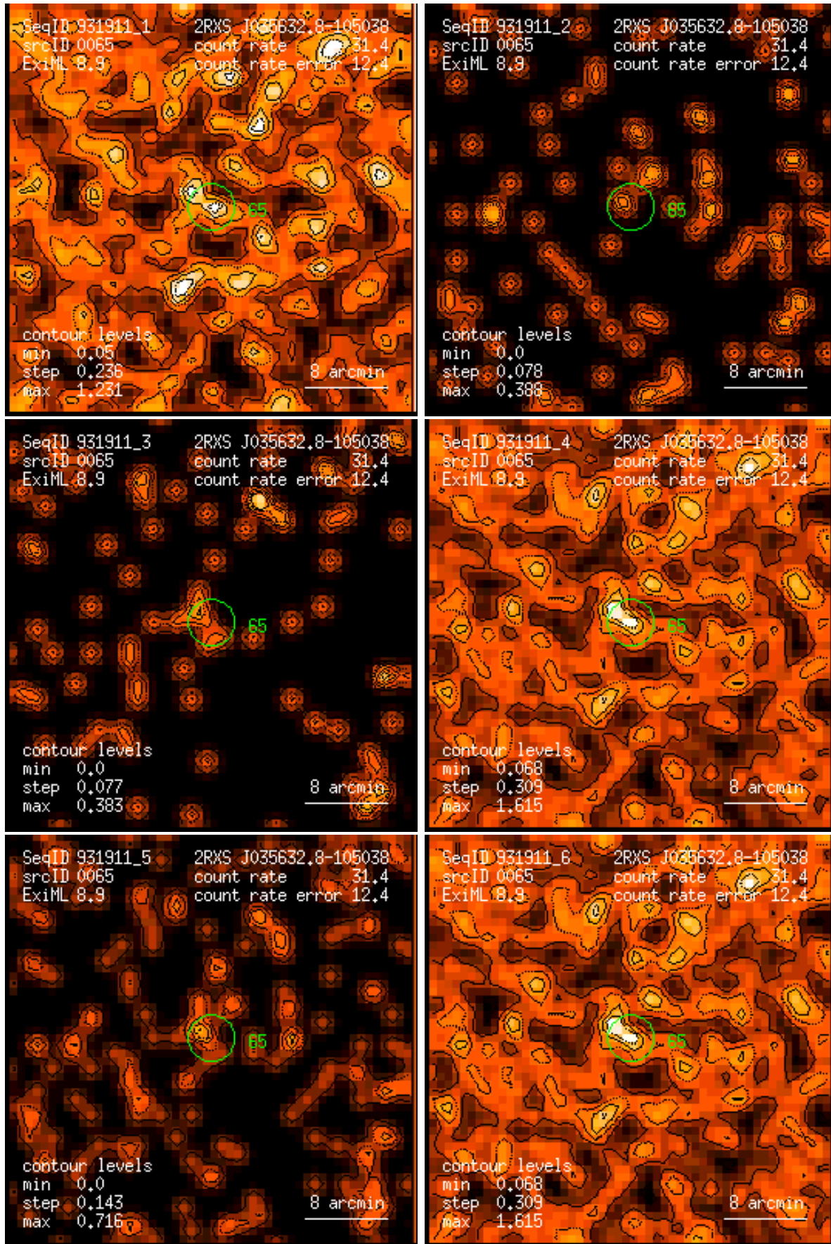
Figure 65: RASS 931911: detection 0065: band rate images, Gaussian filter: (1) PSPC channels 11 – 41, (2) 52 – 90, (3) 91 – 201, (4) 11 – 235, (5) 52 – 201, (6) 11 – 201. Broad band rates in counts/ks. Band rate contour levels in counts/ks/arcmin 2 .
