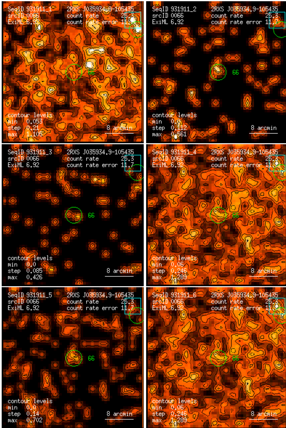
Figure 66: RASS 931911: detection 0066: band rate images, Gaussian filter: (1) PSPC channels 11 – 41, (2) 52 – 90, (3) 91 – 201, (4) 11 – 235, (5) 52 – 201, (6) 11 – 201. Broad band rates in counts/ks. Band rate contour levels in counts/ks/arcmin 2 .
