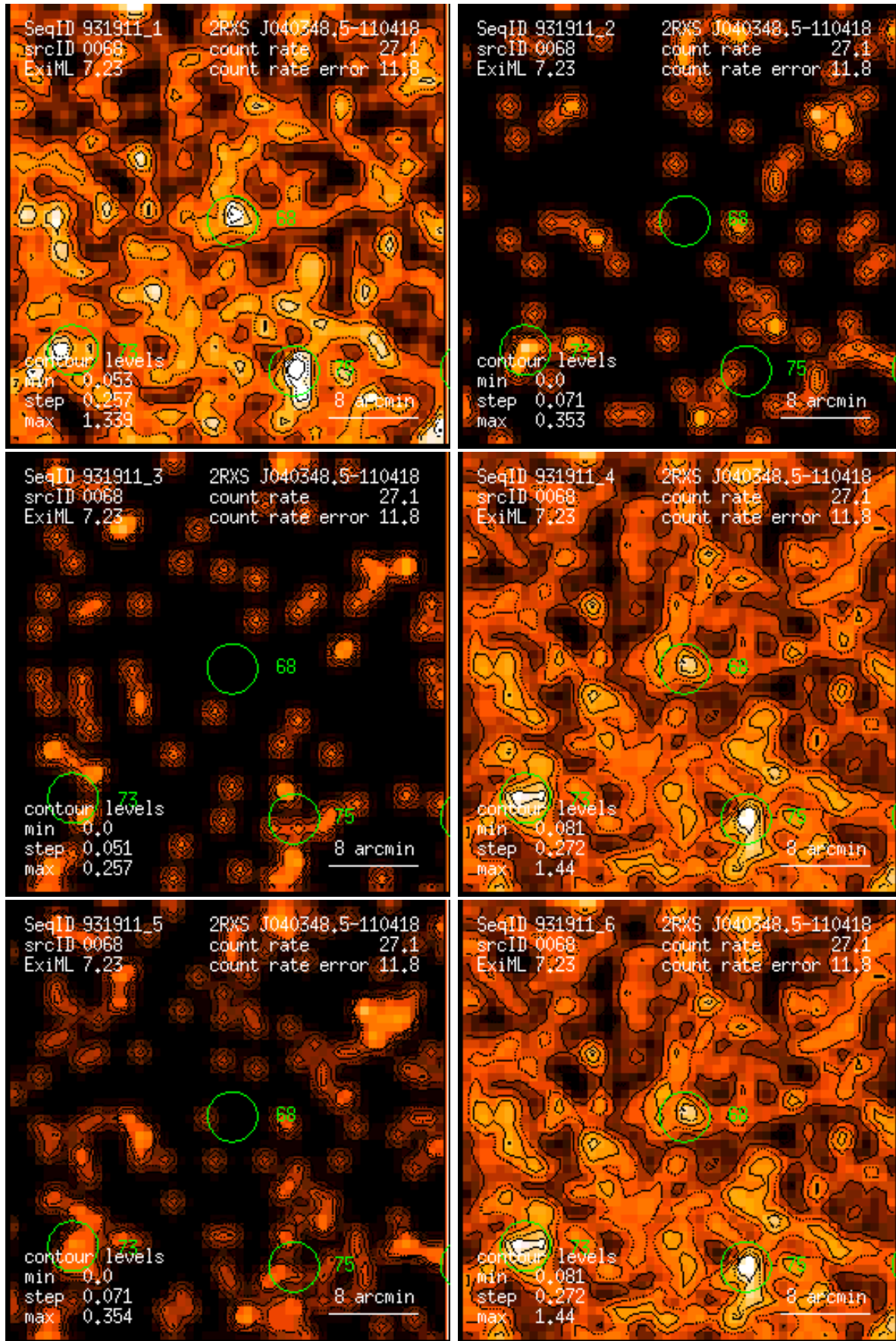
Figure 68: RASS 931911: detection 0068: band rate images, Gaussian filter: (1) PSPC channels 11 – 41, (2) 52 – 90, (3) 91 – 201, (4) 11 – 235, (5) 52 – 201, (6) 11 – 201. Broad band rates in counts/ks. Band rate contour levels in counts/ks/arcmin 2 .
