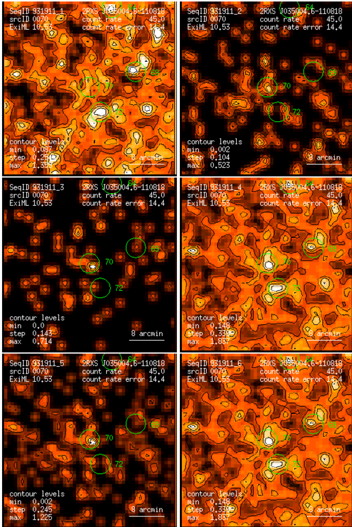
Figure 70: RASS 931911: detection 0070: band rate images, Gaussian filter: (1) PSPC channels 11 – 41, (2) 52 – 90, (3) 91 – 201, (4) 11 – 235, (5) 52 – 201, (6) 11 – 201. Broad band rates in counts/ks. Band rate contour levels in counts/ks/arcmin 2 .
