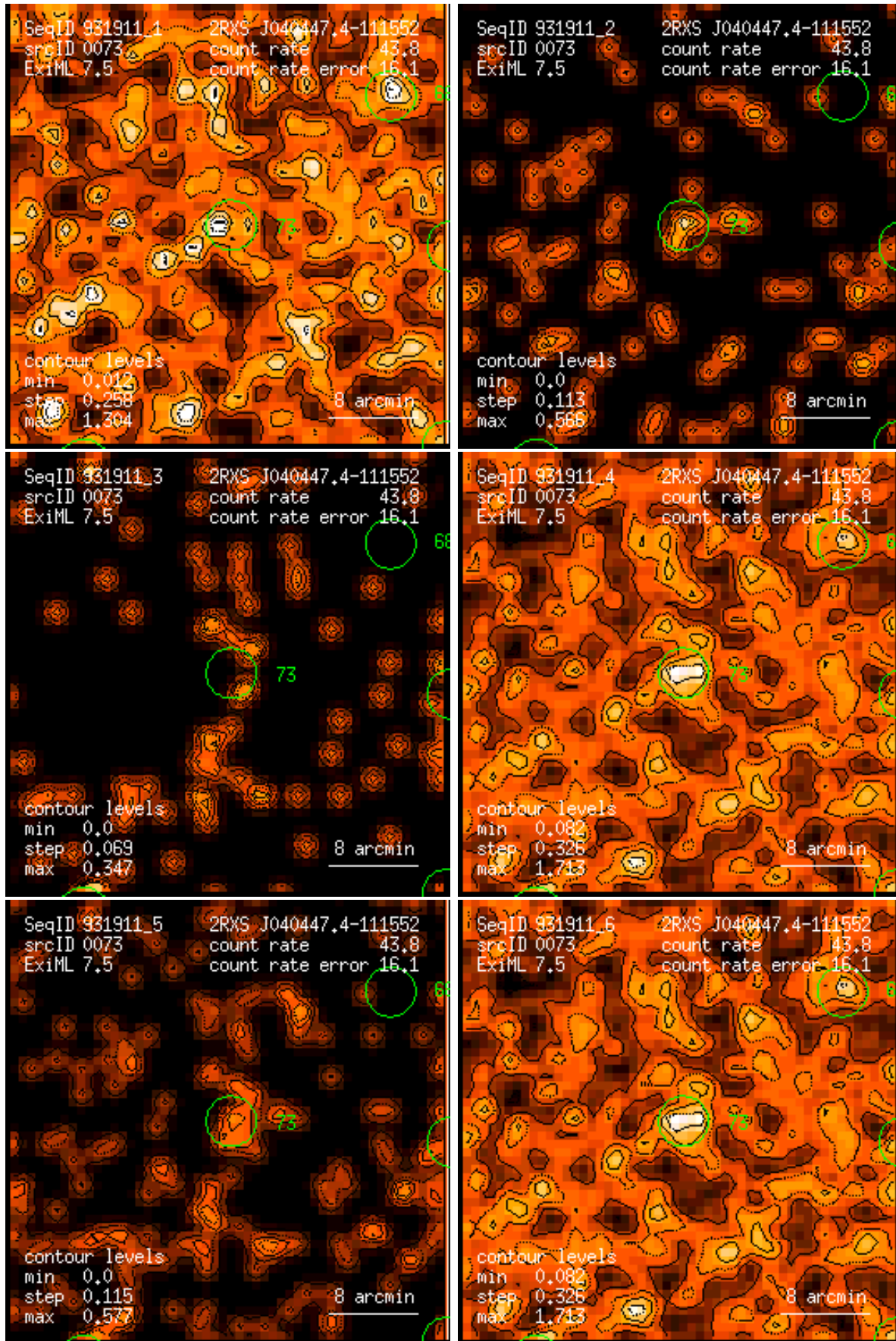
Figure 73: RASS 931911: detection 0073: band rate images, Gaussian filter: (1) PSPC channels 11 – 41, (2) 52 – 90, (3) 91 – 201, (4) 11 – 235, (5) 52 – 201, (6) 11 – 201. Broad band rates in counts/ks. Band rate contour levels in counts/ks/arcmin 2 .
