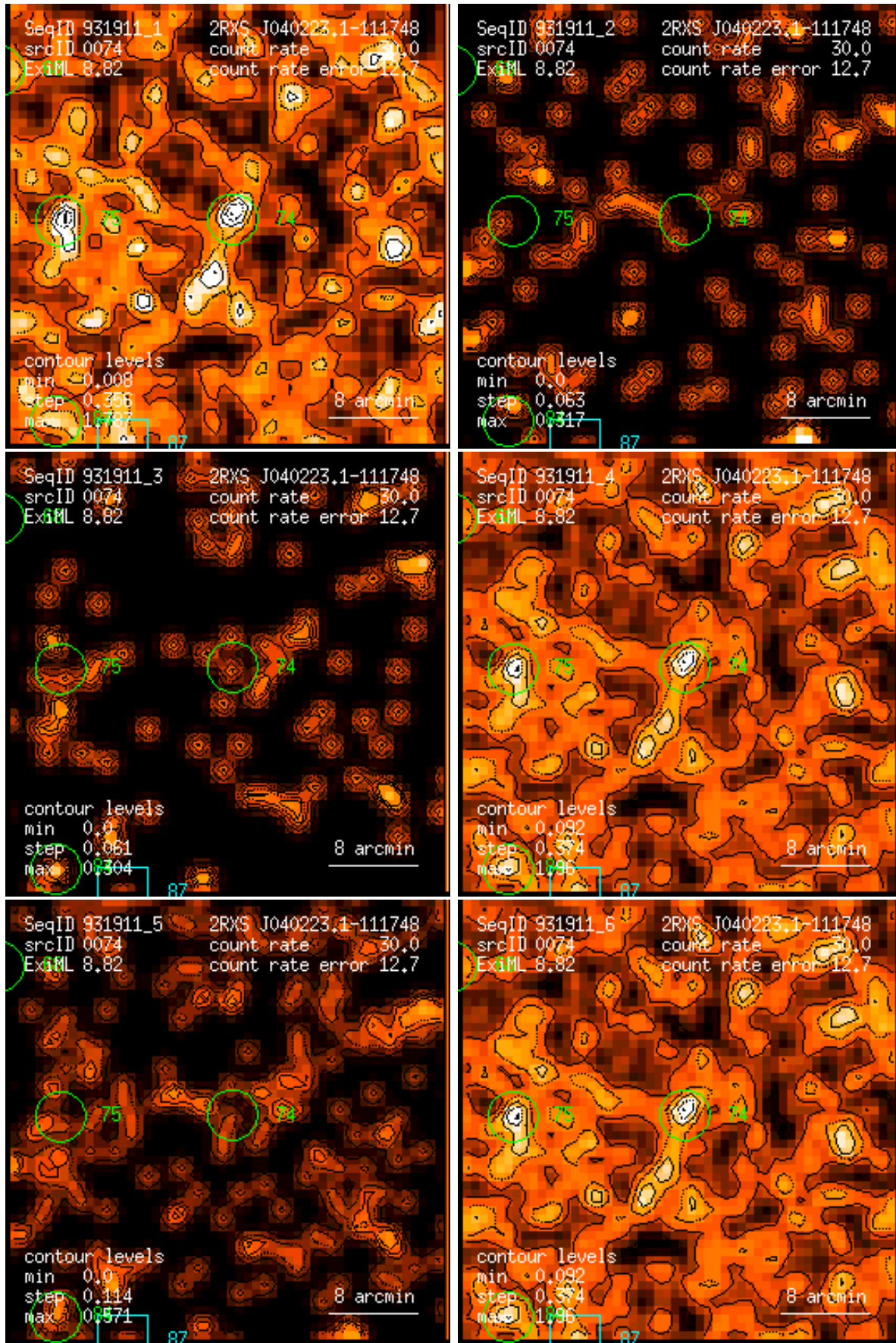
Figure 74: RASS 931911: detection 0074: band rate images, Gaussian filter: (1) PSPC channels 11 – 41, (2) 52 – 90, (3) 91 – 201, (4) 11 – 235, (5) 52 – 201, (6) 11 – 201. Broad band rates in counts/ks. Band rate contour levels in counts/ks/arcmin 2 .
