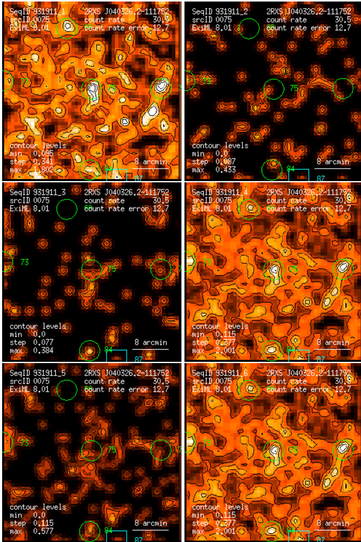
Figure 75: RASS 931911: detection 0075: band rate images, Gaussian filter: (1) PSPC channels 11 – 41, (2) 52 – 90, (3) 91 – 201, (4) 11 – 235, (5) 52 – 201, (6) 11 – 201. Broad band rates in counts/ks. Band rate contour levels in counts/ks/arcmin 2 .
