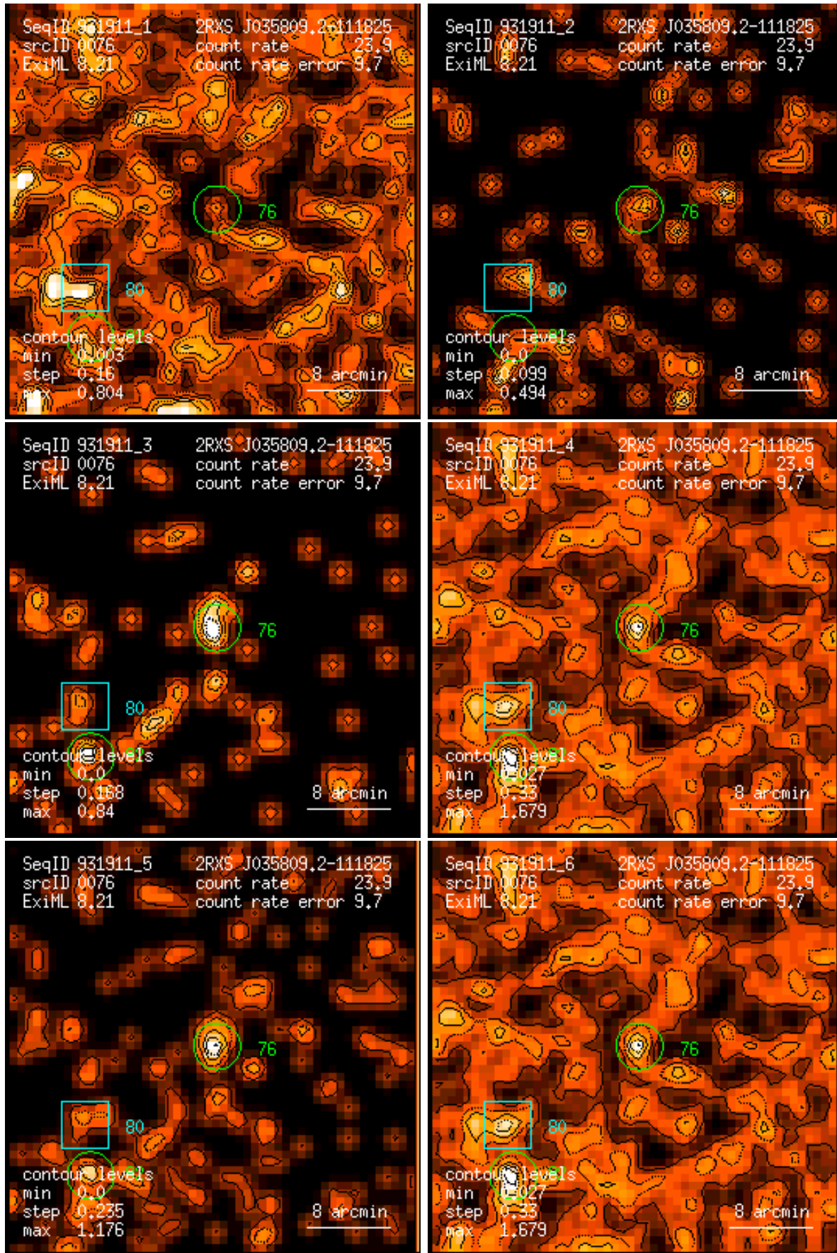
Figure 76: RASS 931911: detection 0076: band rate images, Gaussian filter: (1) PSPC channels 11 – 41, (2) 52 – 90, (3) 91 – 201, (4) 11 – 235, (5) 52 – 201, (6) 11 – 201. Broad band rates in counts/ks. Band rate contour levels in counts/ks/arcmin 2 .
