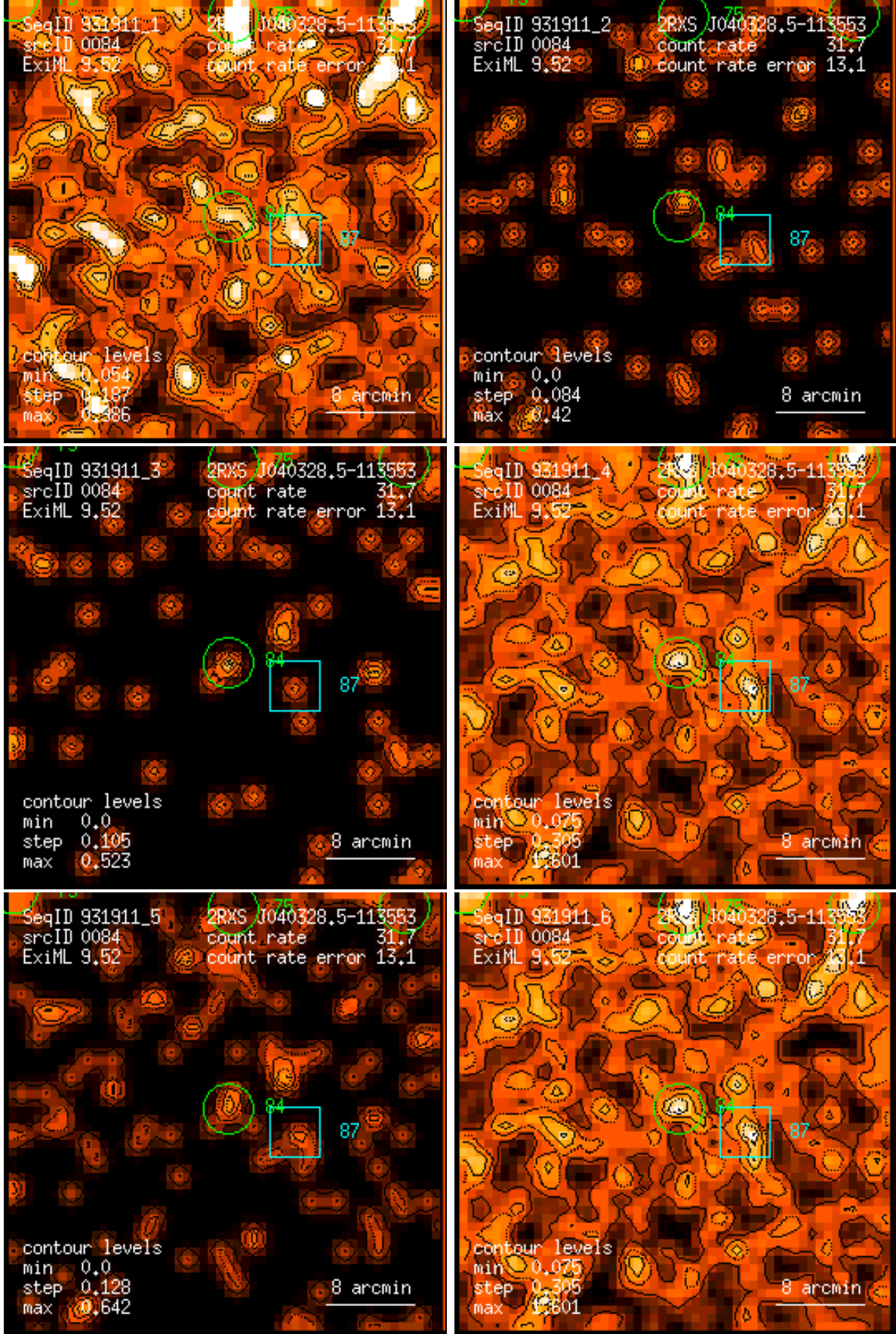
Figure 84: RASS 931911: detection 0084: band rate images, Gaussian filter: (1) PSPC channels 11 – 41, (2) 52 – 90, (3) 91 – 201, (4) 11 – 235, (5) 52 – 201, (6) 11 – 201. Broad band rates in counts/ks. Band rate contour levels in counts/ks/arcmin 2 .
