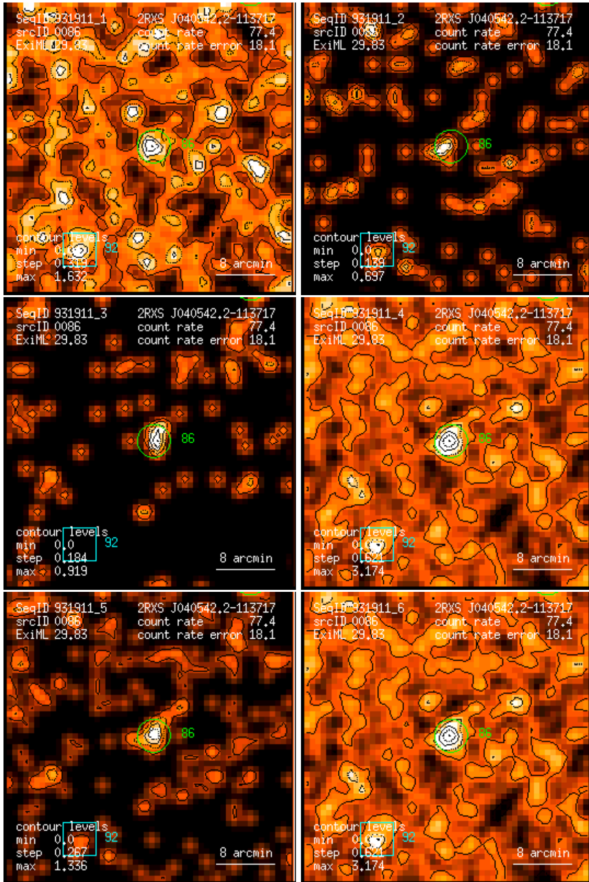
Figure 86: RASS 931911: detection 0086: band rate images, Gaussian filter: (1) PSPC channels 11 – 41, (2) 52 – 90, (3) 91 – 201, (4) 11 – 235, (5) 52 – 201, (6) 11 – 201. Broad band rates in counts/ks. Band rate contour levels in counts/ks/arcmin 2 .
