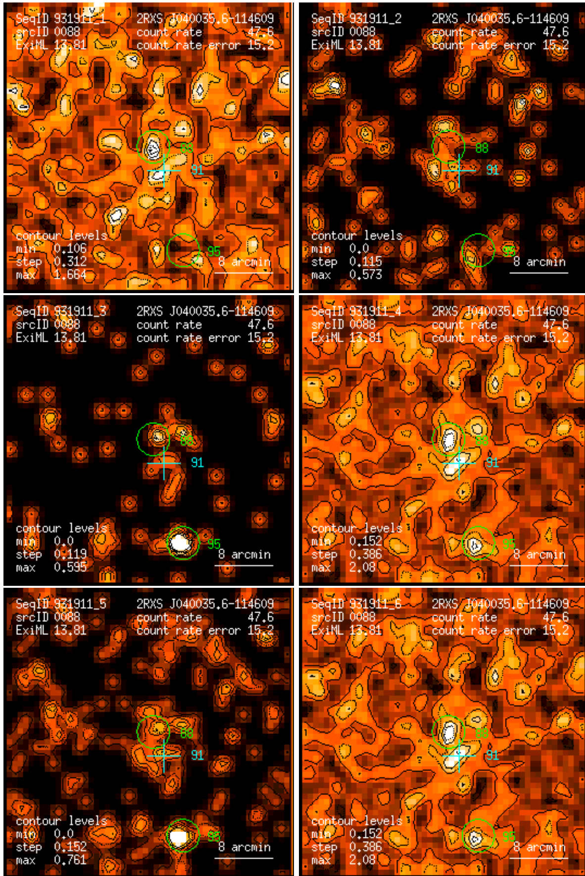
Figure 88: RASS 931911: detection 0088: band rate images, Gaussian filter: (1) PSPC channels 11 – 41, (2) 52 – 90, (3) 91 – 201, (4) 11 – 235, (5) 52 – 201, (6) 11 – 201. Broad band rates in counts/ks. Band rate contour levels in counts/ks/arcmin 2 .
