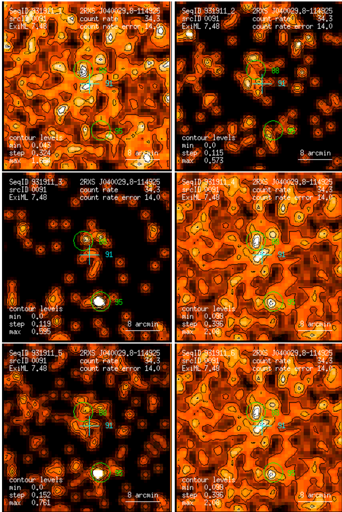
Figure 91: RASS 931911: detection 0091: band rate images, Gaussian filter: (1) PSPC channels 11 – 41, (2) 52 – 90, (3) 91 – 201, (4) 11 – 235, (5) 52 – 201, (6) 11 – 201. Broad band rates in counts/ks. Band rate contour levels in counts/ks/arcmin 2 .
