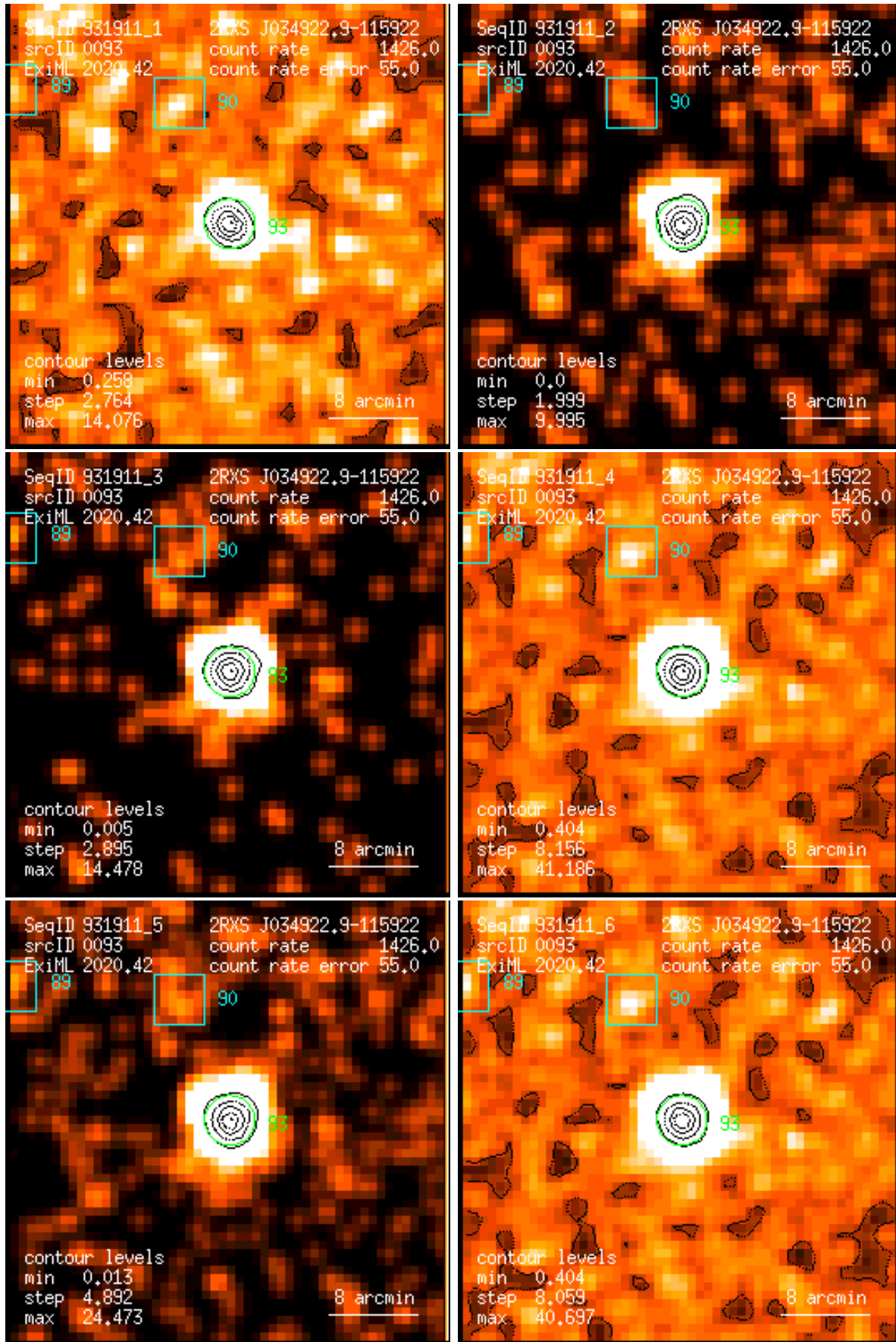
Figure 93: RASS 931911: detection 0093: band rate images, Gaussian filter: (1) PSPC channels 11 – 41, (2) 52 – 90, (3) 91 – 201, (4) 11 – 235, (5) 52 – 201, (6) 11 – 201. Broad band rates in counts/ks. Band rate contour levels in counts/ks/arcmin 2 .
