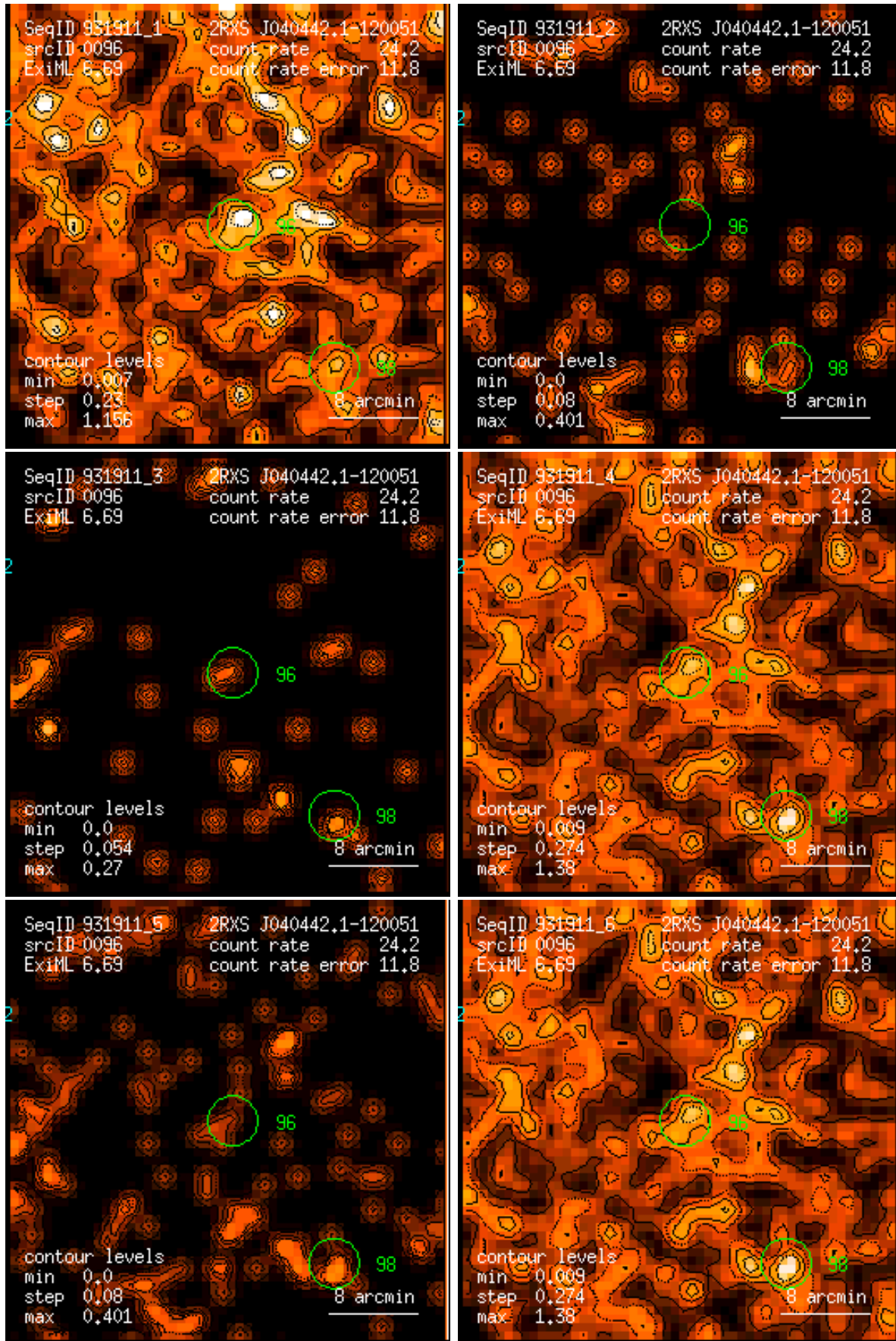
Figure 96: RASS 931911: detection 0096: band rate images, Gaussian filter: (1) PSPC channels 11 – 41, (2) 52 – 90, (3) 91 – 201, (4) 11 – 235, (5) 52 – 201, (6) 11 – 201. Broad band rates in counts/ks. Band rate contour levels in counts/ks/arcmin 2 .
