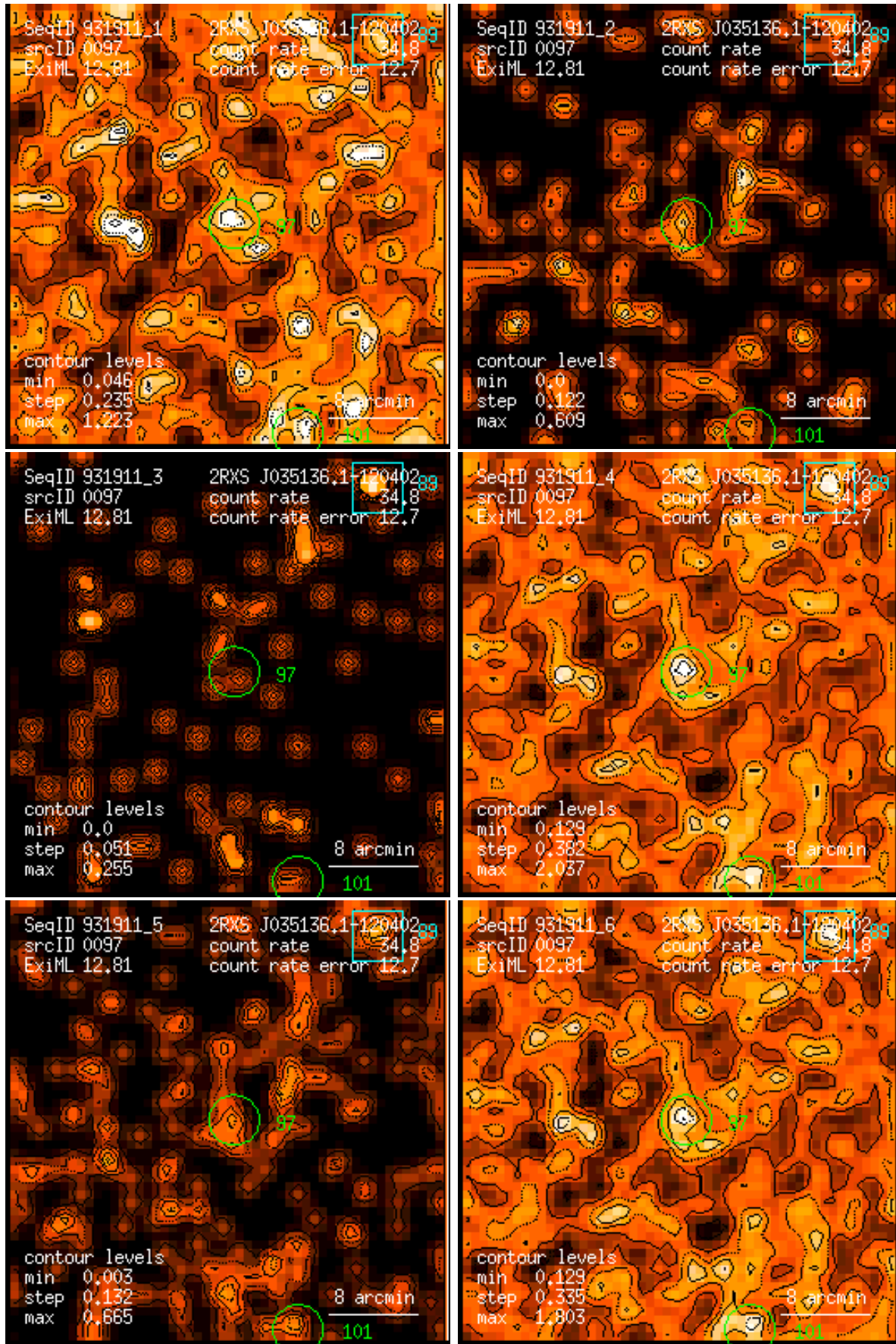
Figure 97: RASS 931911: detection 0097: band rate images, Gaussian filter: (1) PSPC channels 11 – 41, (2) 52 – 90, (3) 91 – 201, (4) 11 – 235, (5) 52 – 201, (6) 11 – 201. Broad band rates in counts/ks. Band rate contour levels in counts/ks/arcmin 2 .
