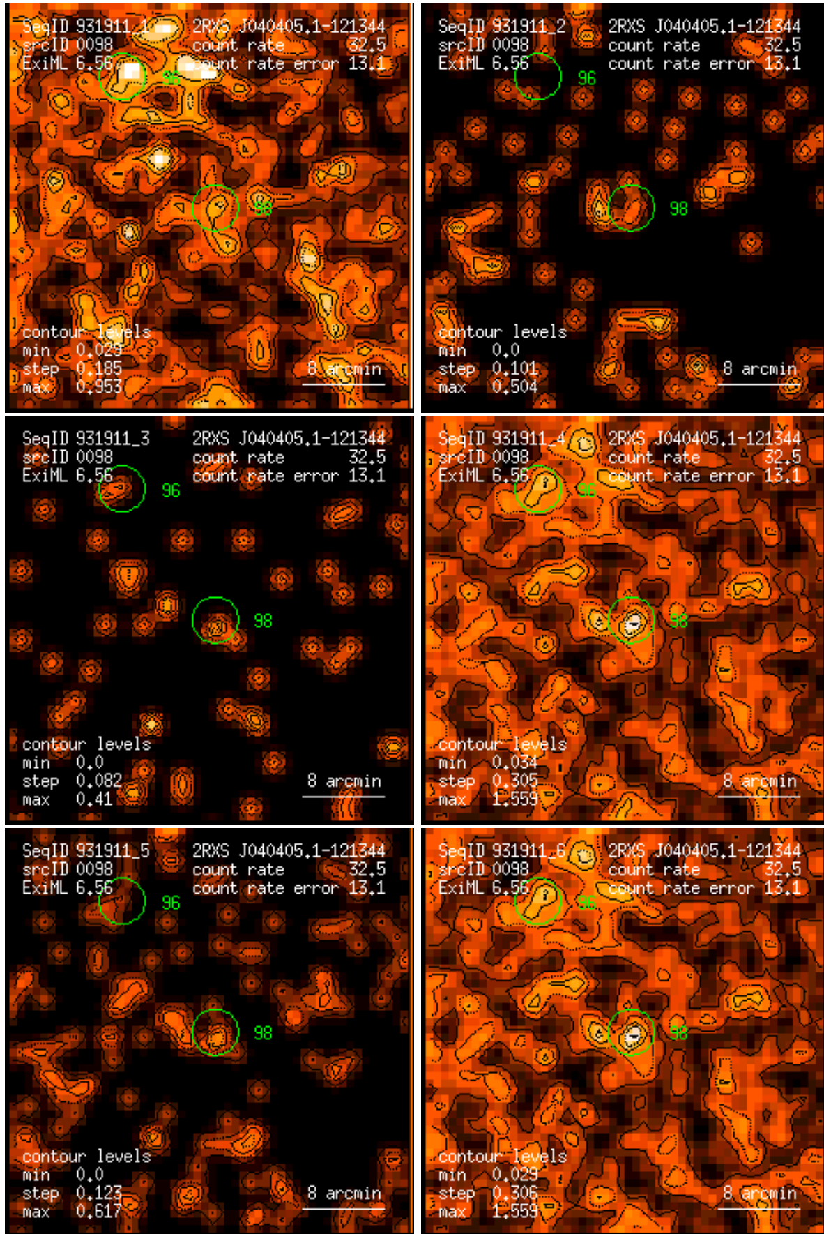
Figure 98: RASS 931911: detection 0098: band rate images, Gaussian filter: (1) PSPC channels 11 – 41, (2) 52 – 90, (3) 91 – 201, (4) 11 – 235, (5) 52 – 201, (6) 11 – 201. Broad band rates in counts/ks. Band rate contour levels in counts/ks/arcmin 2 .
