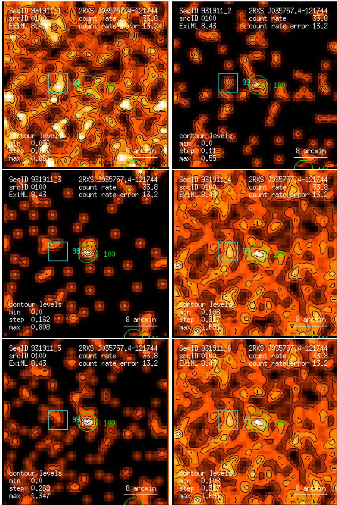
Figure 100: RASS 931911: detection 0100: band rate images, Gaussian filter: (1) PSPC channels 11 – 41, (2) 52 – 90, (3) 91 – 201, (4) 11 – 235, (5) 52 – 201, (6) 11 – 201. Broad band rates in counts/ks. Band rate contour levels in counts/ks/arcmin 2 .
