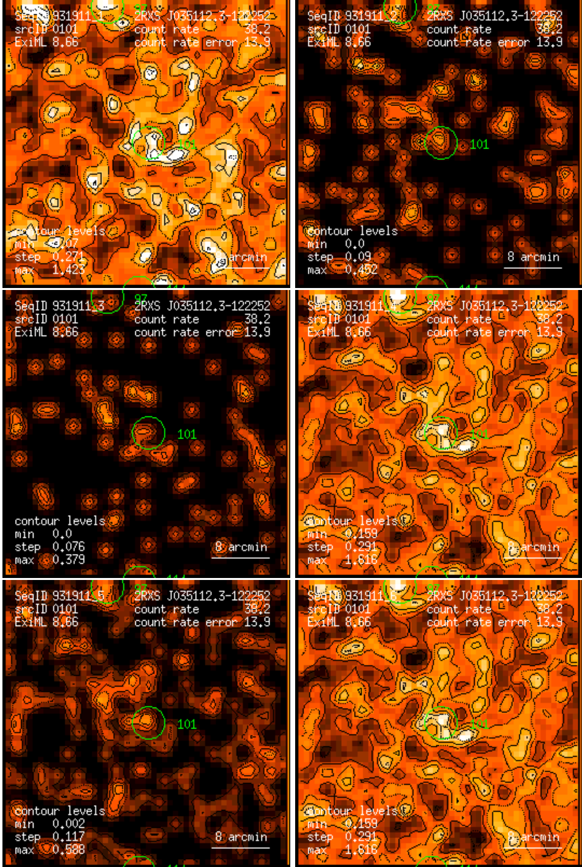
Figure 101: RASS 931911: detection 0101: band rate images, Gaussian filter: (1) PSPC channels 11 – 41, (2) 52 – 90, (3) 91 – 201, (4) 11 – 235, (5) 52 – 201, (6) 11 – 201. Broad band rates in counts/ks. Band rate contour levels in counts/ks/arcmin 2 .
